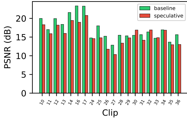
Figure 5: Per-clip PSNR for baseline and speculative decoding on 20 clips. Speculation incurs a mean PSNR drop of 1.54 dB.
