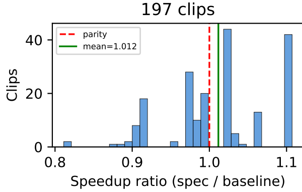
Figure 4: Per-clip speedup ratio (speculative / baseline) over 197 paired clips. The mean is 1.012\times ; speculation is faster on 53.3% of clips.
