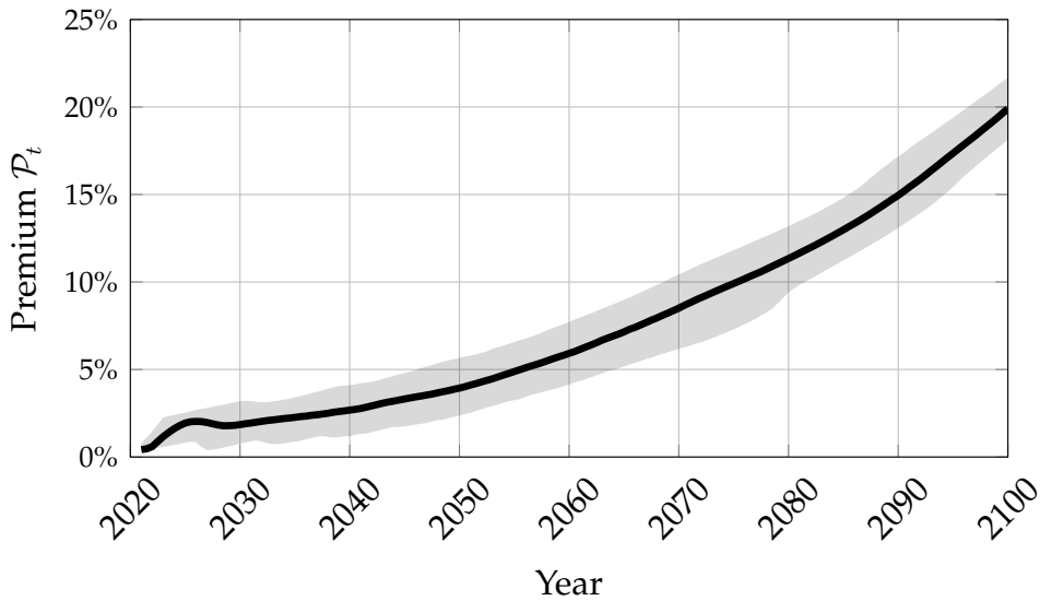
Figure 15: Median and 95% simulation intervals of the uncertainty premium \mathcal{P}_t (35) of 100,000 simulations. The simulation is conditional on temperature T_t not crossing the critical threshold T_t^{c,*} .
