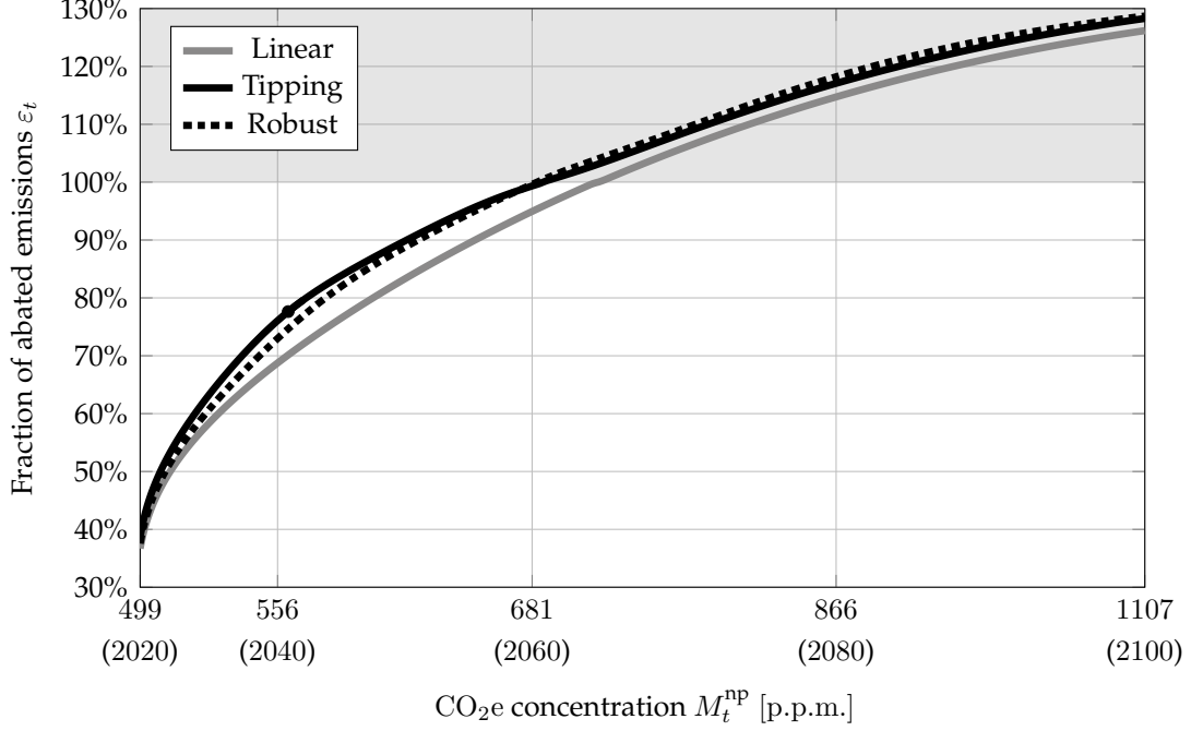
Figure 14: Median optimal abated fraction of emissions \varepsilon_t along the no-policy path of \text{CO}_2\text{e} concentration M_t^{np} of 100,000 simulations using the optimal policy \bar{\varphi} in a linear climate (grey), \varphi^{T^c} in a tipping climate (black), and the robust policy \varphi^r (dashed). The marker represents the \text{CO}_2\text{e} concentration at which the no-policy np temperature T is at the critical threshold T^c = 2.5^\circ of the tipping climate. The shaded area represents negative emissions.
