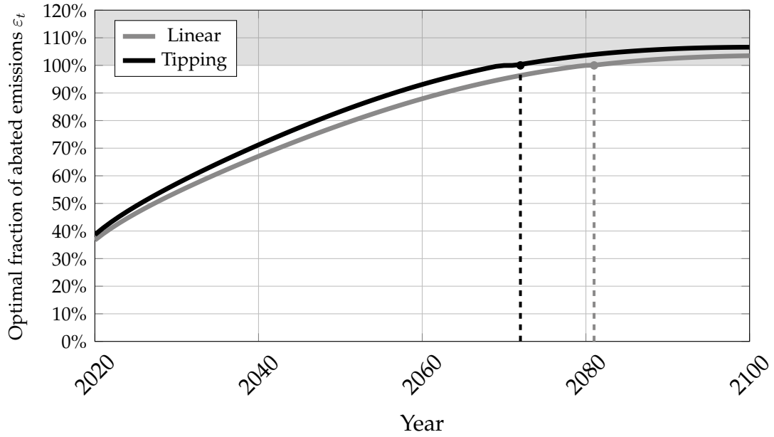
Figure 7: Median optimal abated fraction of emissions \varepsilon_t at time t of 100,000 simulations in a linear (grey) and a tipping climate (black).
