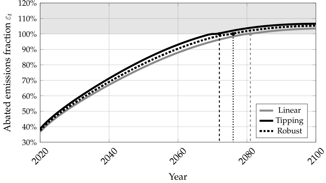
Figure 12: Median optimal abated fraction of emissions \varepsilon_t over time t of 100,000 simulations using the optimal policy in a linear climate (grey), in a tipping climate (black), and the robust policy (dashed).
