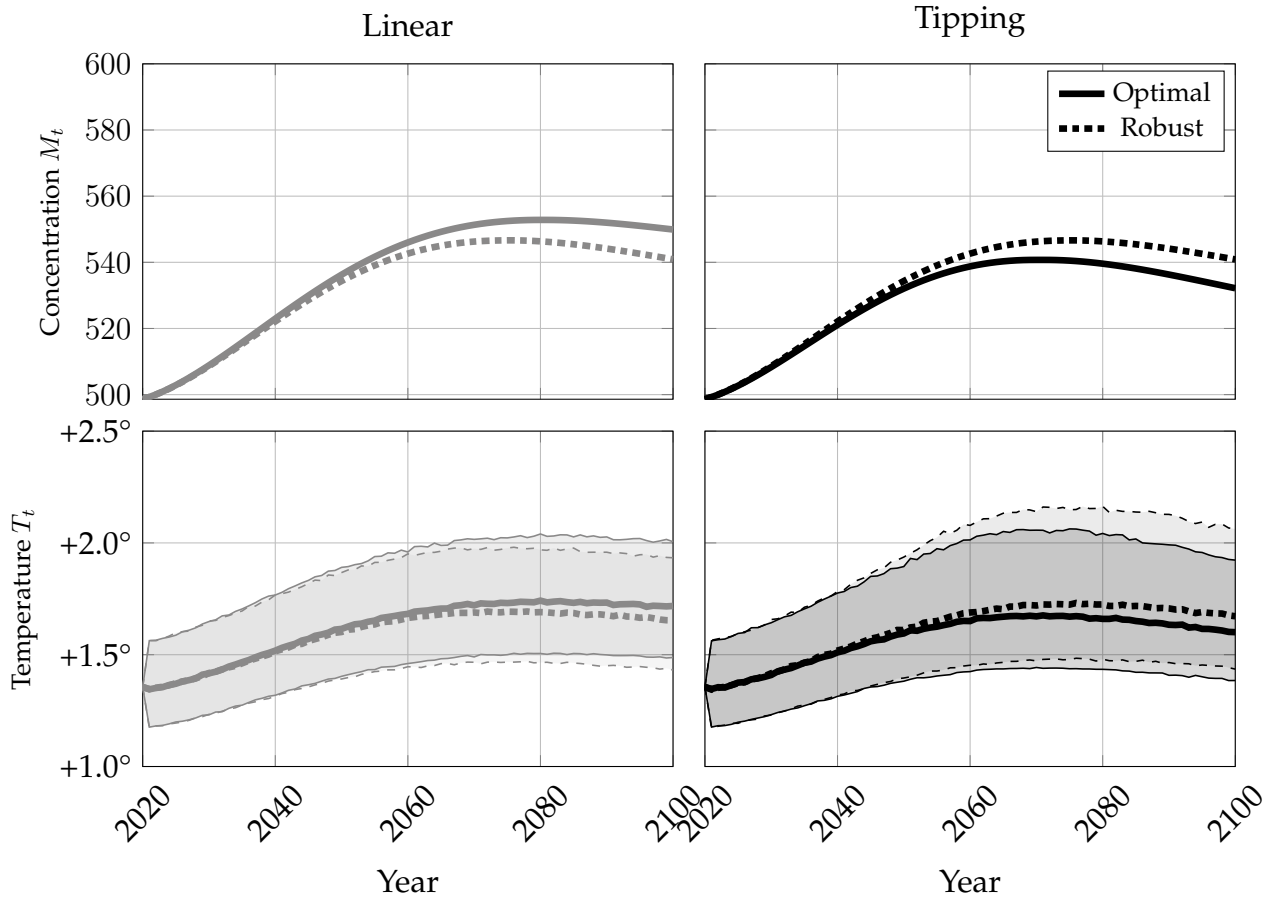
Figure 13: Median and 95% simulation intervals of CO 2 e concentration M_t (ppm, top row) and temperature T_t (bottom row) over time t of 100,000 simulations in a linear climate (left column) and a tipping climate (right column). Solid lines and darker shaded bands show the optimal policy \varphi^{T^c} ; dash-dotted lines and lighter shaded bands show the robust policy \varphi^r . The dashed horizontal lines in the temperature panels indicate the critical threshold T^c .
