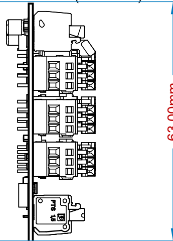
View from Left side (Scale 1:1)
