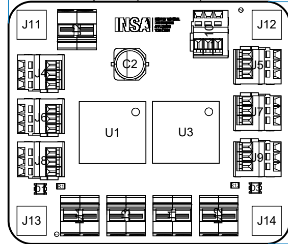
View from Top side (Scale 1:1)
