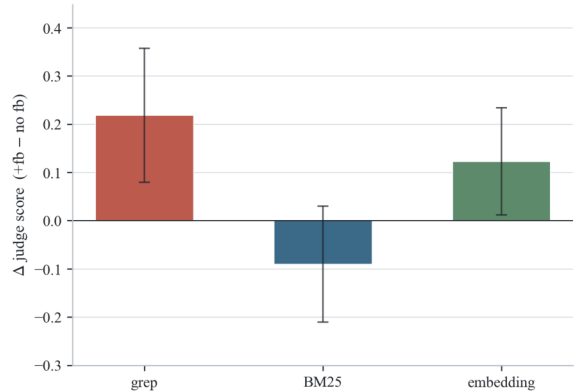
Figure 1: The effect of applying process-level LLM-as-a-Judge feedback to Agentic retrieval. We observe significant difference in performance gains across various retrieval modules. Simple grep retrieval benefits from the provided feedback the most, BM25 does not show any improvement at all, while embedding-model based retrieval shows intermediate gains.
