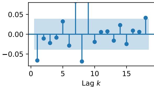
AAPL log returns: PACF
