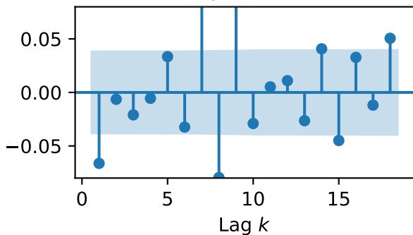
AAPL log returns: ACF
