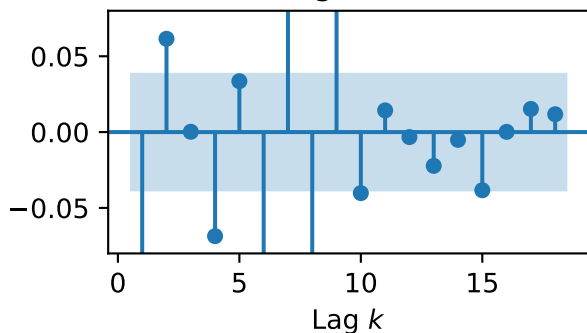
S&P 500 log returns: PACF
