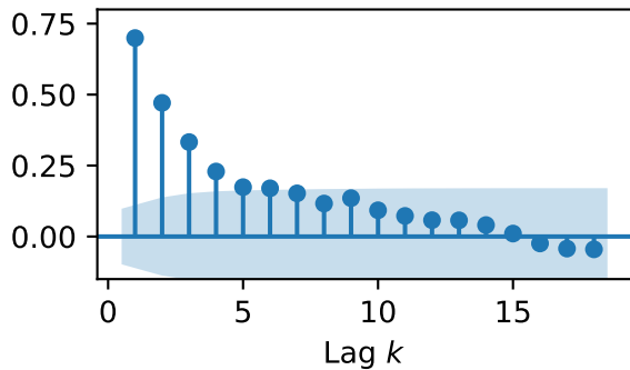
Simulated AR(1), \phi_1 = 0.7 : ACF
