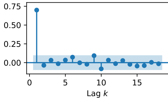
Simulated AR(1), \phi_1 = 0.7 : PACF
