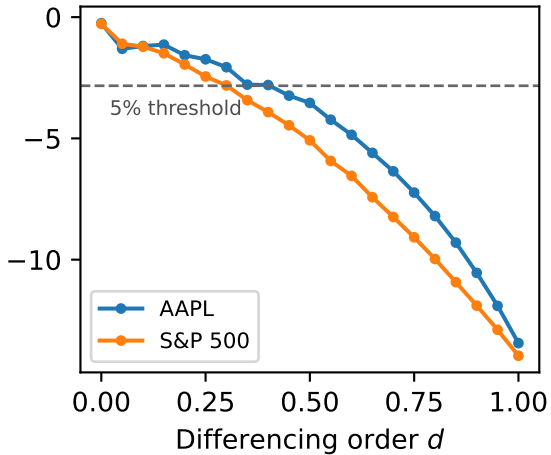
Stationarity against differencing order
