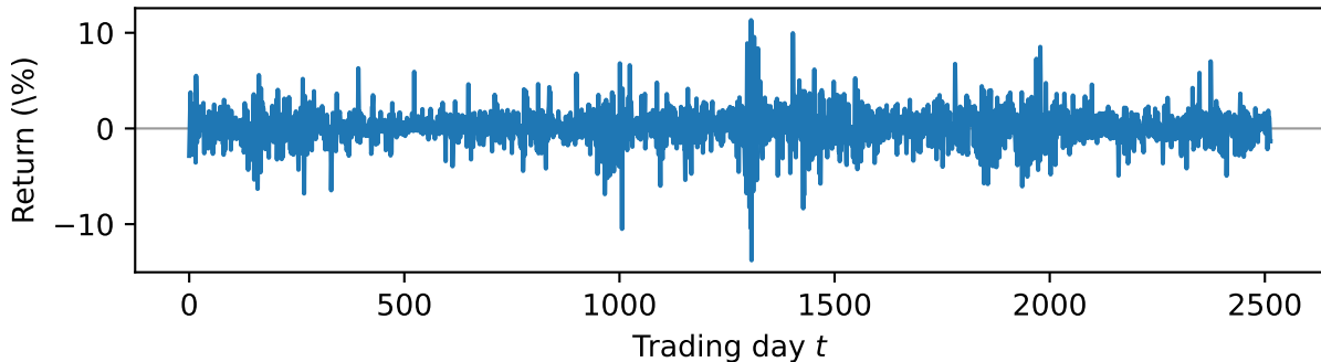
First difference \Delta \ln X_t (ADF t = -13.44 )
