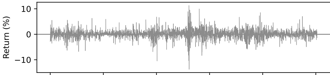
AAPL daily returns
