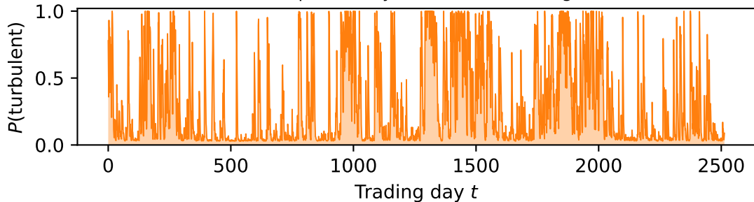
Filtered probability of the turbulent regime
