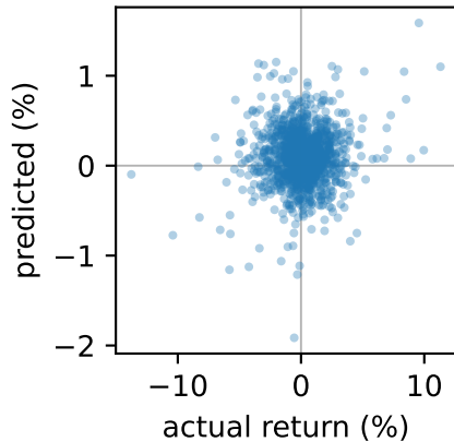
correlation +0.101
