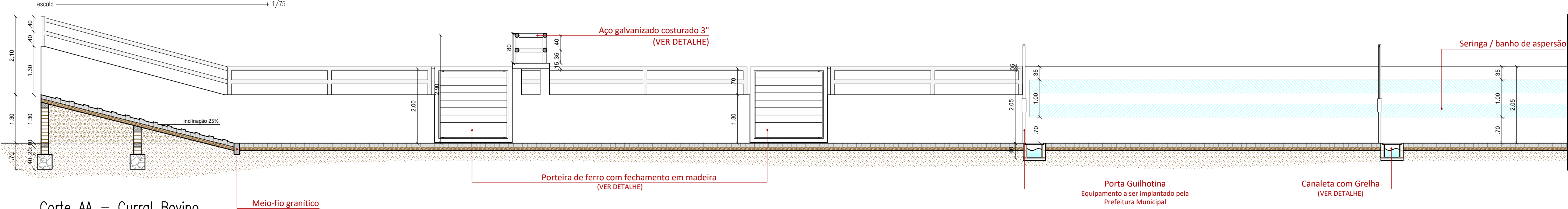
Corte AA – Curral Bovino
