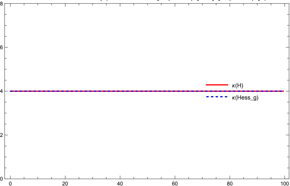
Condition Number vs \xi (Quadratic L=x^2+4y^2 )
