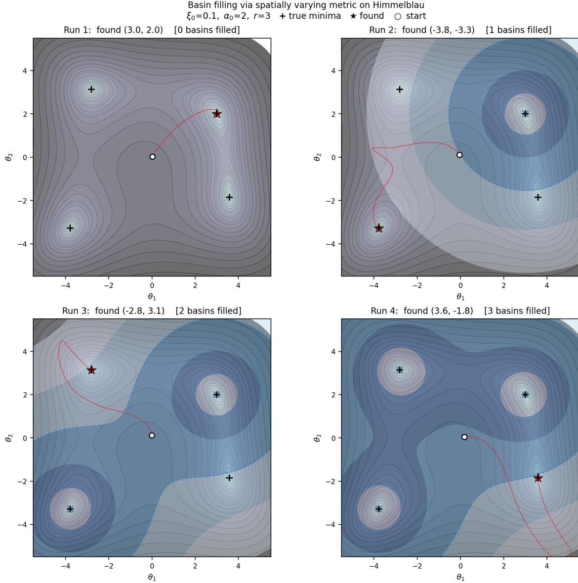
Figure 6: Progressive basin filling on Himmelblau’s function. Each panel shows one optimiser run (red trajectory from ○ to ★) on the loss contours (grey). Blue shading shows the damping field 1 - \Phi(\theta) : regions where \xi(\theta) \rightarrow 0 and the gradient-norm clipping is removed. Run 1 discovers the first minimum with no prior basins. Runs 2–4 start from the same initial point but are deflected by the modified metric, discovering a new minimum each time. All four global minima are found in four runs.
