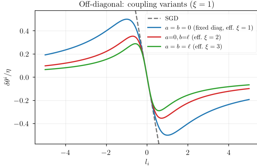
Figure 3: Step-size profiles for off-diagonal variants in 1D ( \xi = 1 ). The one-sided and symmetric couplings provide progressively stronger damping compared to the fixed diagonal baseline (effective \xi of 2 and 3 respectively).
