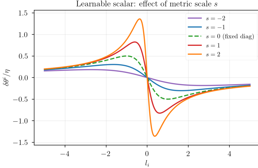
Figure 2: Step-size profile for the learnable scalar metric ( \xi = 1 ). Increasing s amplifies the peak step size and shifts it toward smaller gradients; decreasing s flattens the curve, approaching plain SGD. The dashed line is the fixed diagonal baseline ( s = 0 ).
