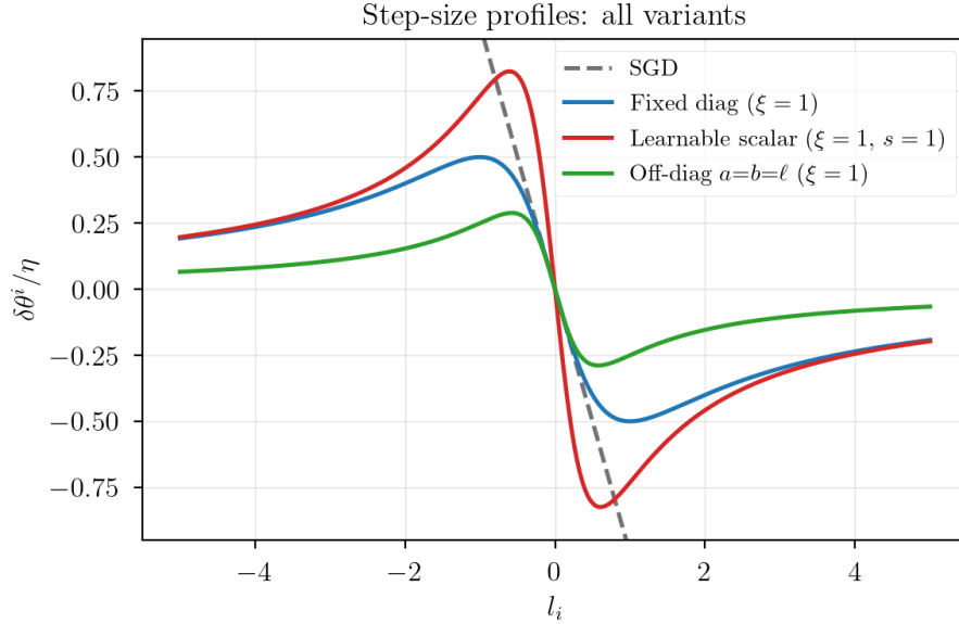
Figure 4: Step-size profiles compared across all variants ( \xi = 1 ). All induced-metric optimisers exhibit smooth gradient clipping relative to SGD. The learnable scalar ( s = 1 ) has a larger peak step size but clips at the same rate; the off-diagonal symmetric coupling clips more aggressively.
