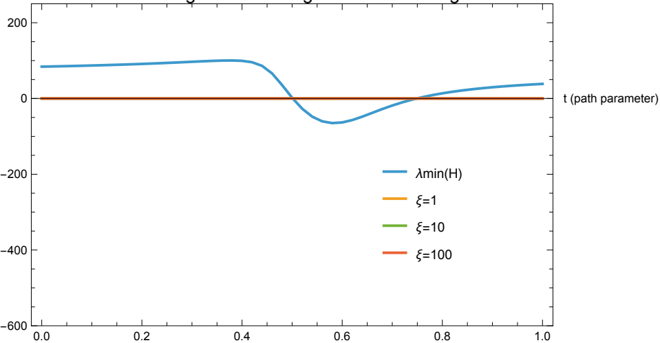
Minimum Eigenvalue Along Rosenbrock Diagonal
