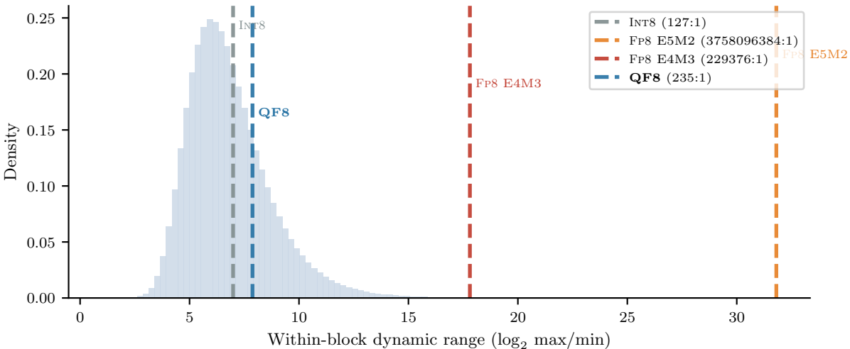
Weight dynamic range per block vs. format capacity
