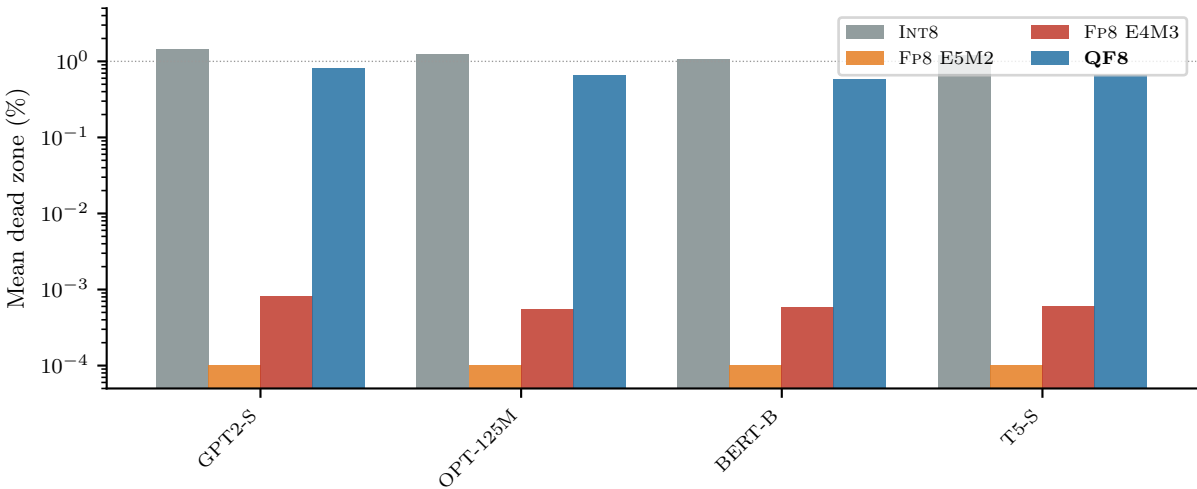
Fraction of nonzero weights rounded to zero per block
