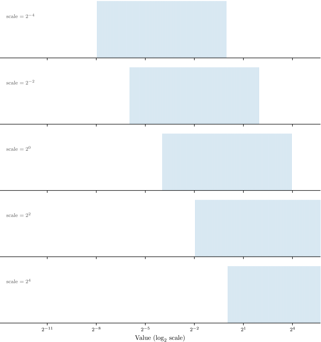
QF8 + E8M0 block scale
