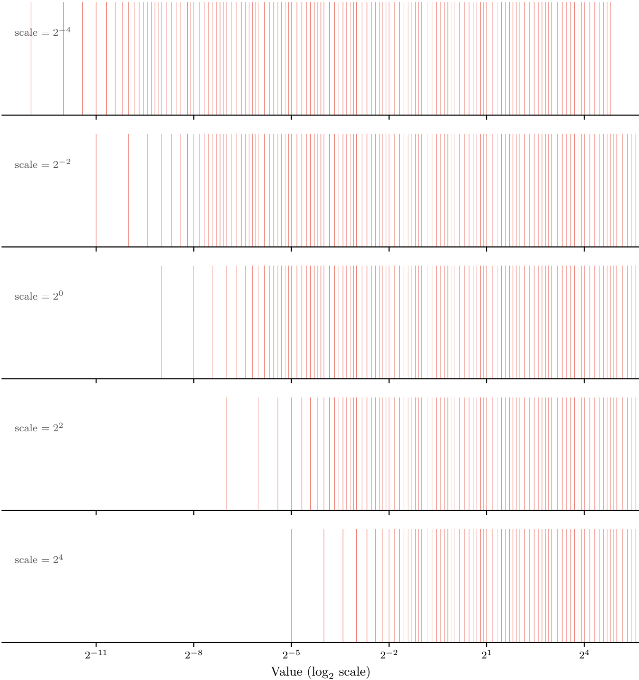
FP8 E4M3 + E8M0 block scale
