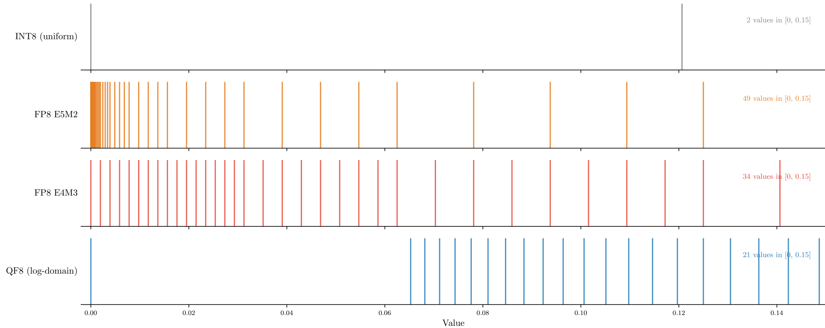
Representable Numbers Near Zero (positive half, [0, 0.15] )
