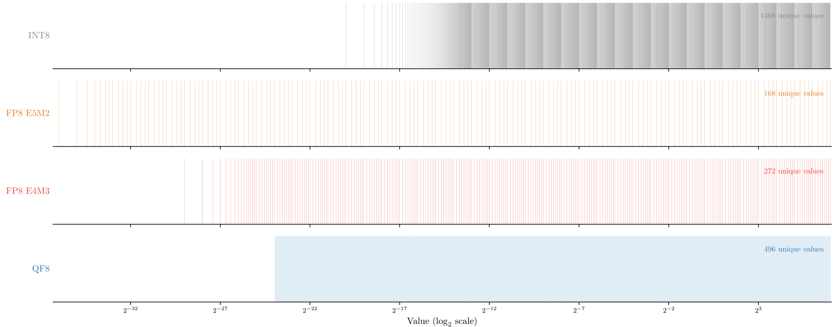
All Representable Numbers in [0, 128] — Union Across All E8M0 Scales ( \log_2 )
