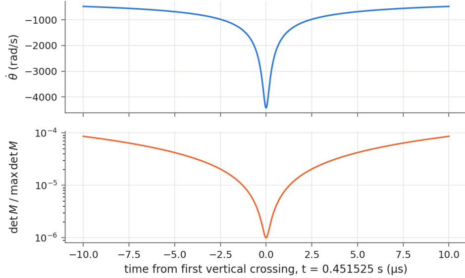
Figure 3: Angular velocity, and determinant of the mass matrix relative to its maximum, in the 20 \mu s around the first vertical crossing. The spike has a peak of 4,429 rad/s and a full width at half maximum of 1.08 \mu s; at 10 \mu s from the crossing |\dot{\theta}| is still about 477 rad/s. The same event recurs at every crossing.
