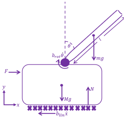
Figure 2.1: Simplified model of the inverted pendulum system showing the generalized coordinates, pendulum angle, and input force.
