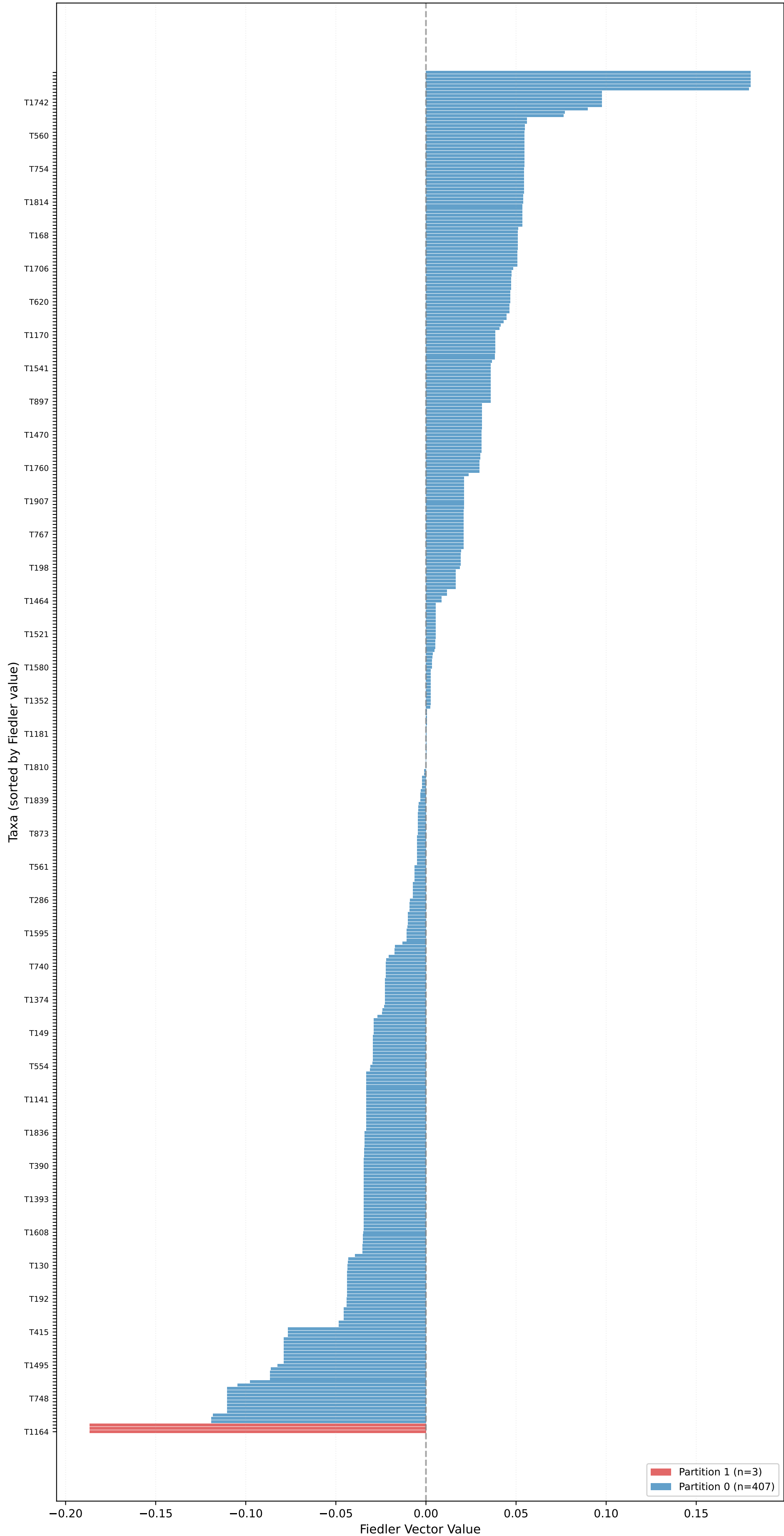
Partition for extinction_heavy (n=2000, L=10000, \mu=0.20 ) - Fiedler Vector \sigma_2=0.0000 , Gap=0.0000, Coherence=0.2331
