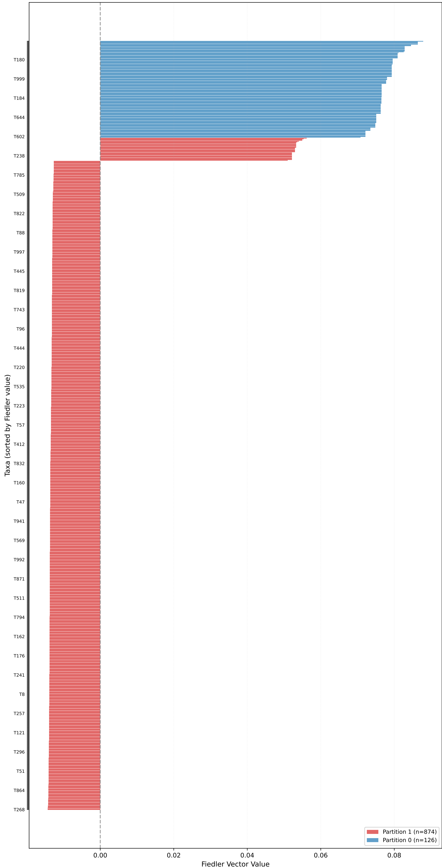
Partition for kingman_mean_pop_0.1 (n=1000, L=10000, \mu=0.10 ) - Fiedler Vector \sigma_2=0.0264 , Gap=13.3567, Coherence=0.0060
