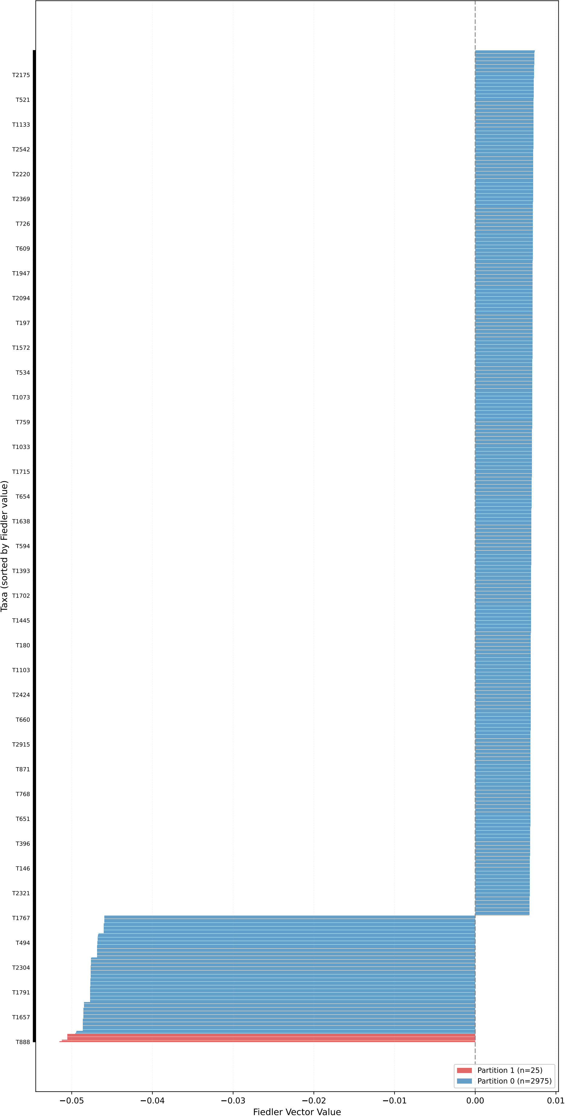
Partition for kingman_mean_pop_0.1 (n=3000, L=10000, \mu=0.10 ) - Fiedler Vector \sigma_2=0.0158 , Gap=53.9361, Coherence=0.0023
