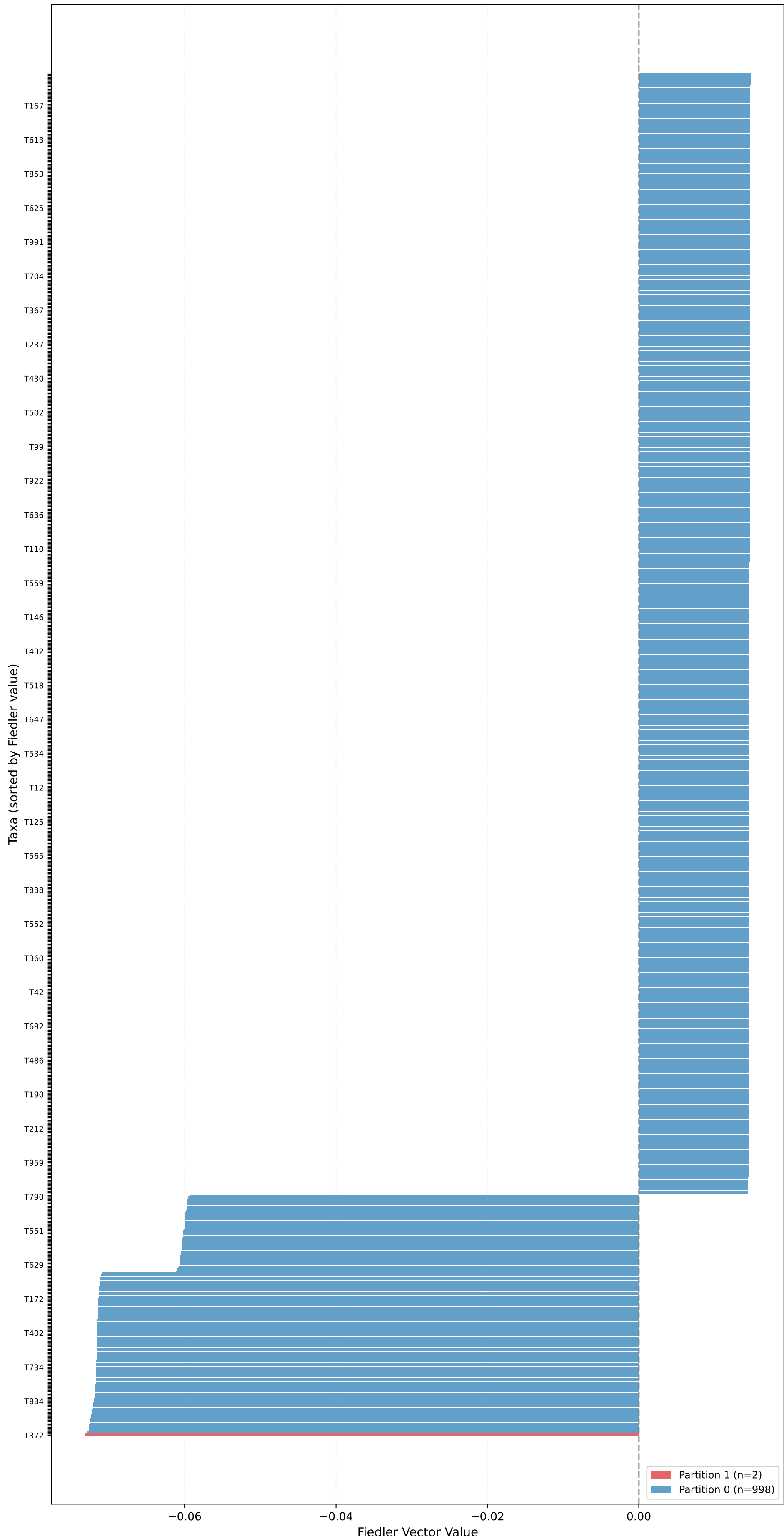
Partition for kingman_mean_pop_1 (n=1000, L=10000, \mu=0.10 ) - Fiedler Vector \sigma_2=0.0000 , Gap=45.9908, Coherence=0.0070
