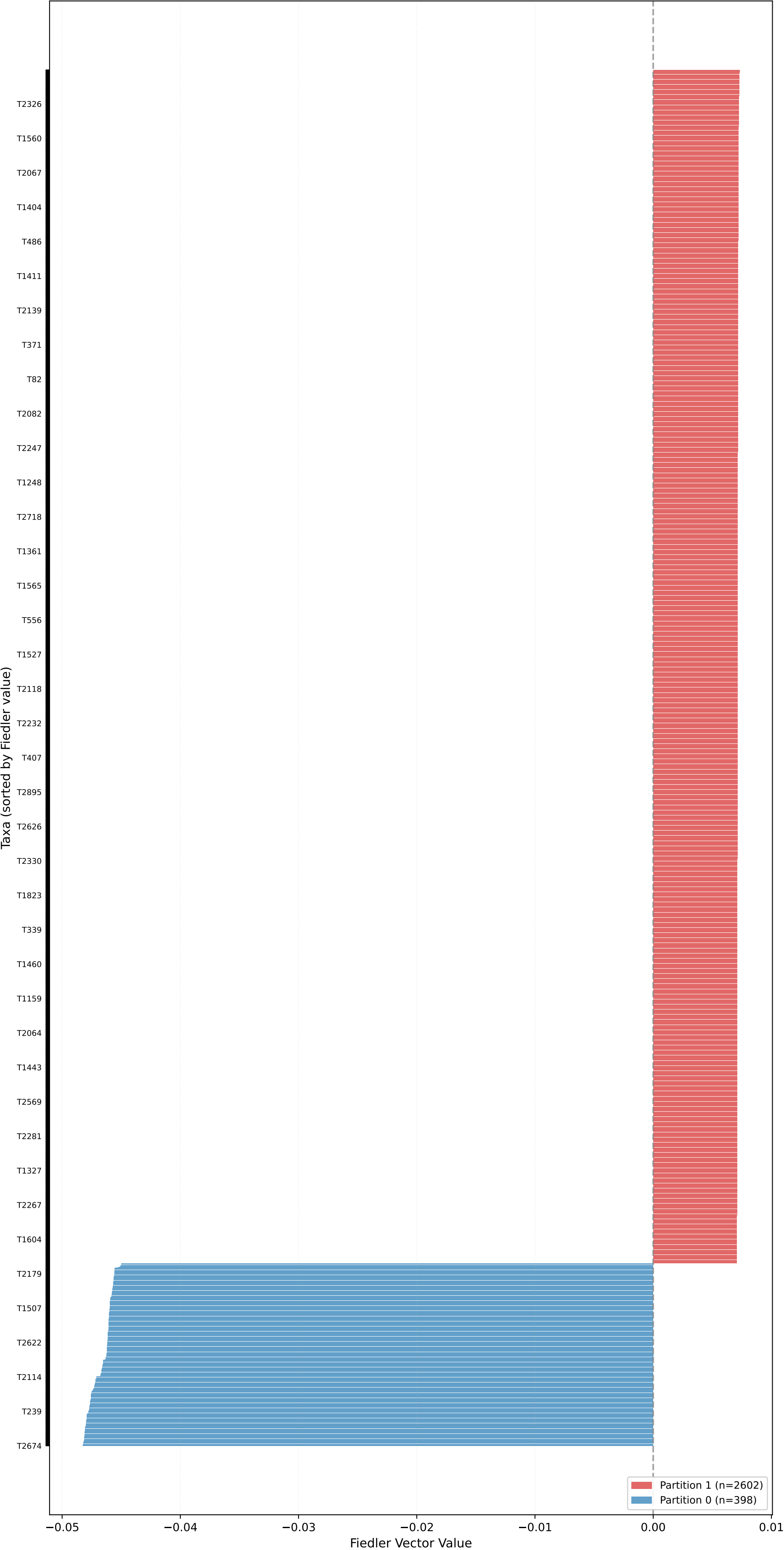
Partition for kingman_mean_pop_1 (n=3000, L=10000, \mu=0.10 ) - Fiedler Vector \sigma_2=0.4232 , Gap=250.3145, Coherence=0.0025
