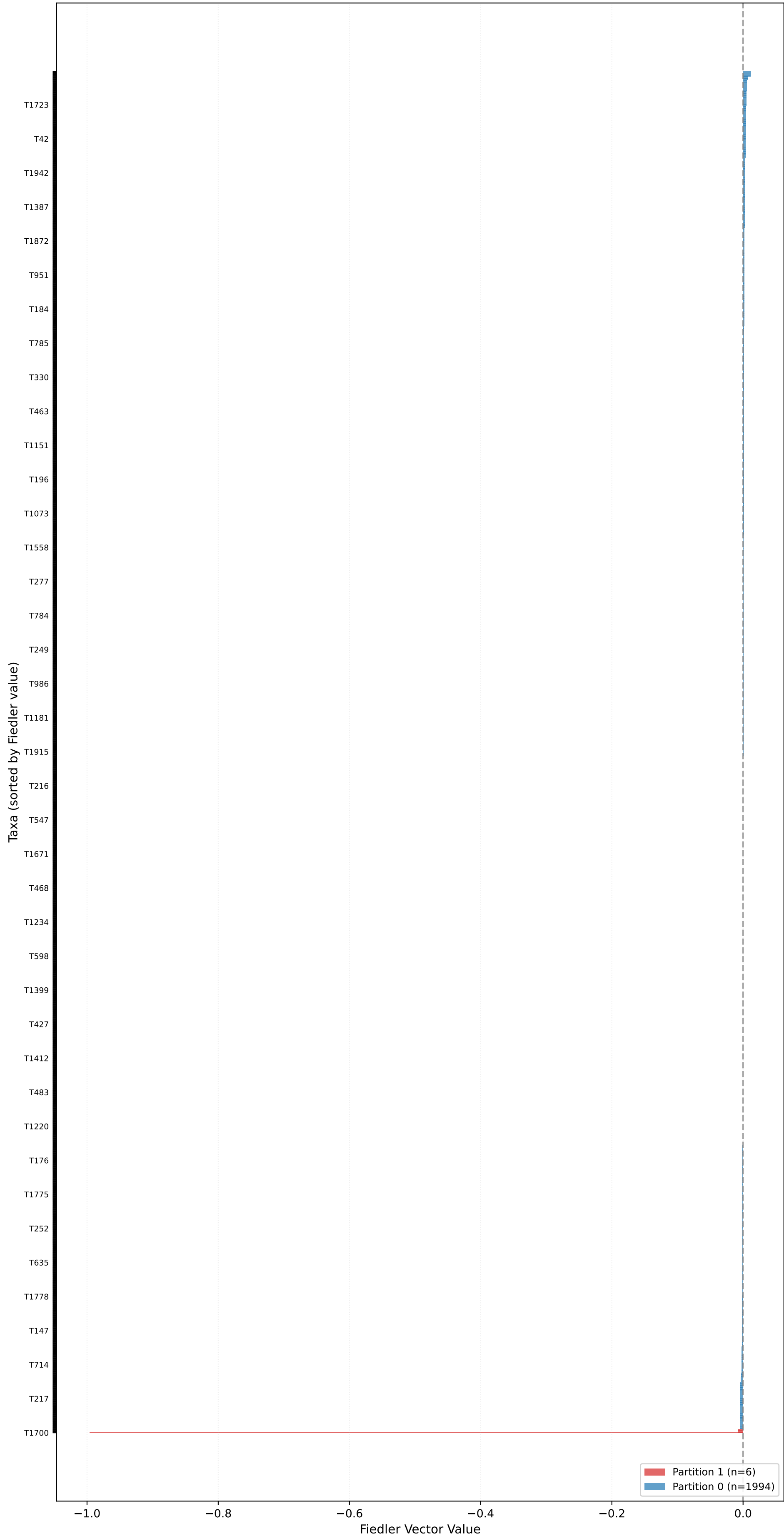
Partition for kingman_mean_pop_1000 (n=2000, L=10000, \mu=0.10 ) - Fiedler Vector \sigma_2=0.0000 , Gap=0.0000, Coherence=0.0575
