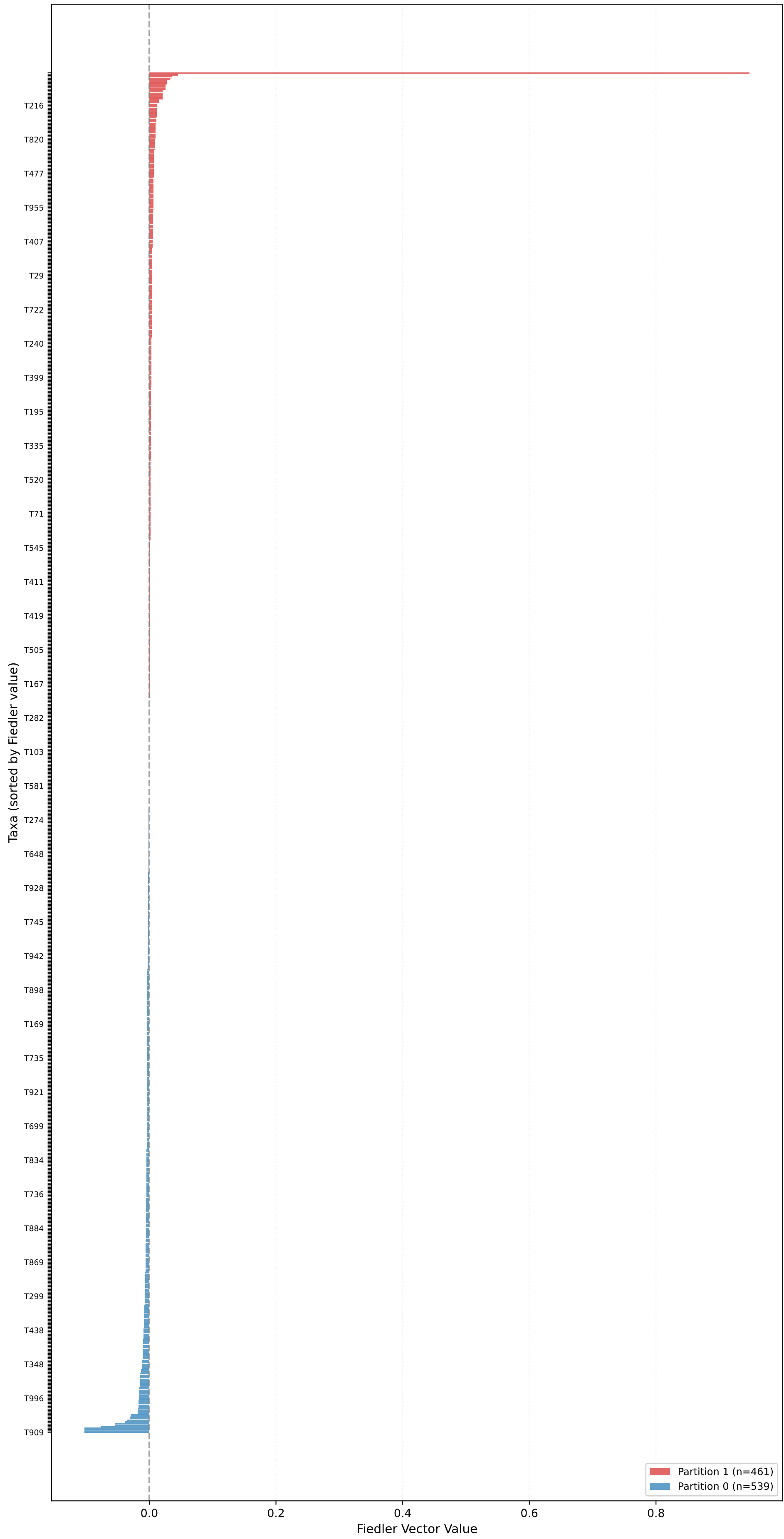
Partition for unrooted_pure_kingman_tree_pop_size_1000 (n=1000, L=10000, \mu=0.20 ) - Fiedler Vector \sigma_2=0.0001 , Gap=0.0000, Coherence=0.2313
