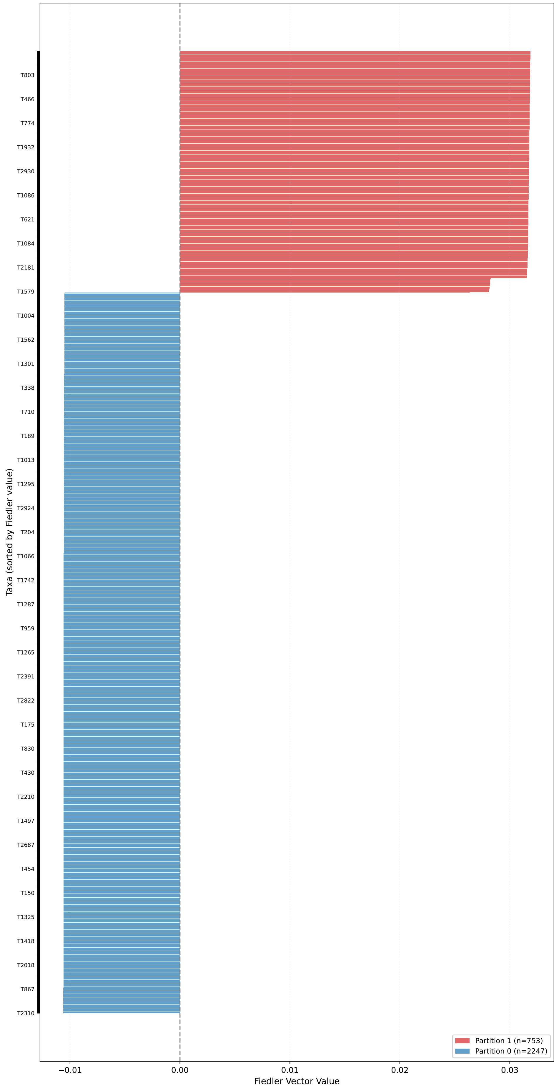
Partition for unrooted_kingman_tree_pop_size_1.0 (n=3000, L=10000, \mu=0.20 ) - Fiedler Vector \sigma_2=0.4174 , Gap=85.3477, Coherence=0.0017
