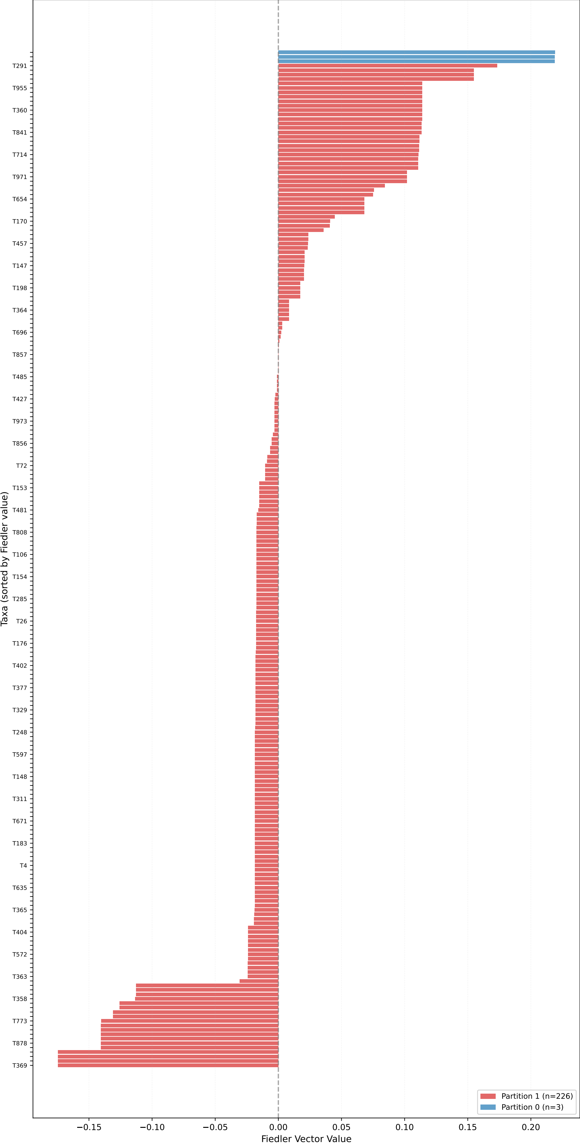
Partition for extinction_heavy (n=1000, L=10000, \mu=0.20 ) - Fiedler Vector \sigma_2=0.0000 , Gap=0.0000, Coherence=0.1770
