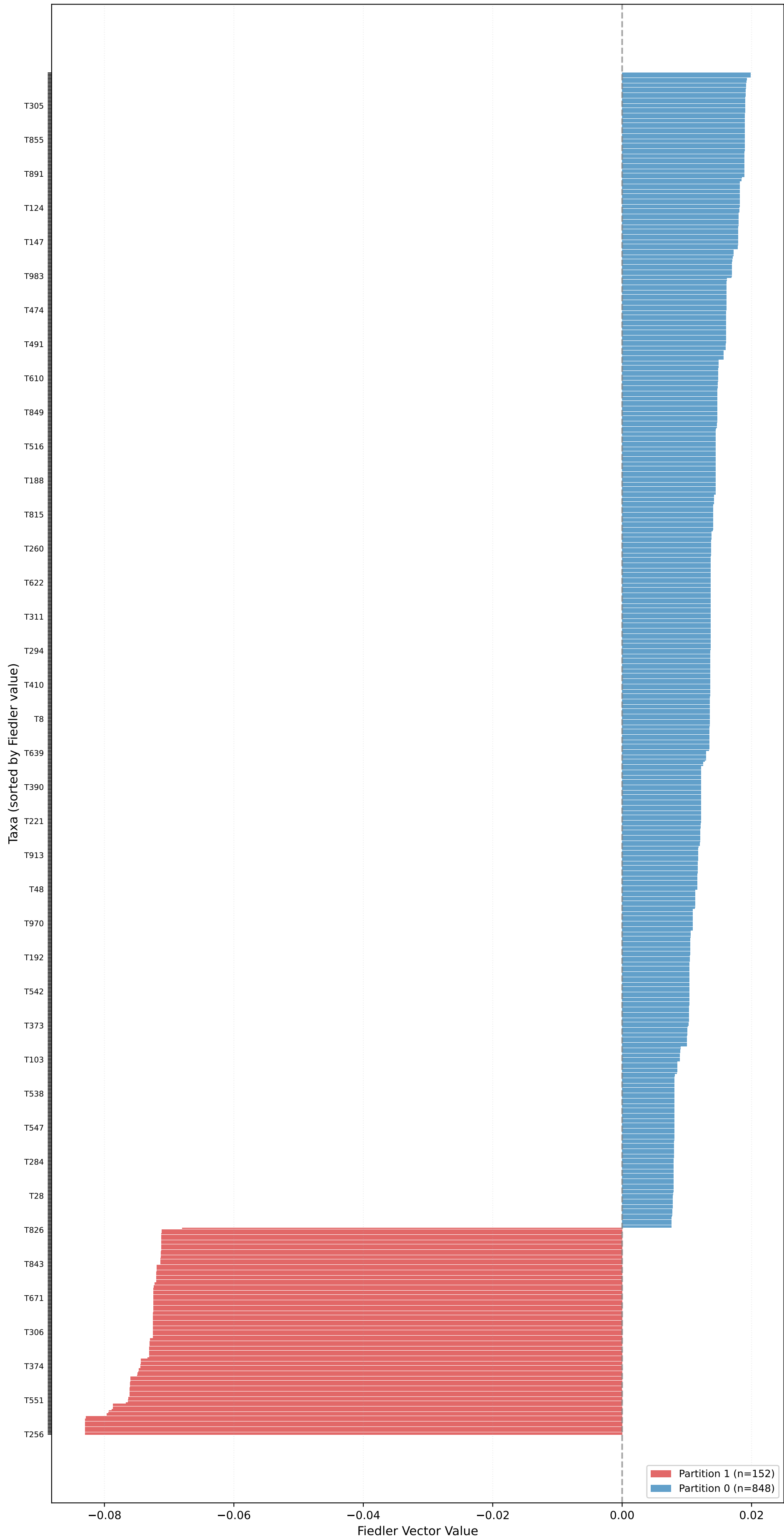
Partition for yule_pure_birth (n=1000, L=10000, \mu=0.20 ) - Fiedler Vector \sigma_2=0.0001 , Gap=0.0000, Coherence=0.1902
