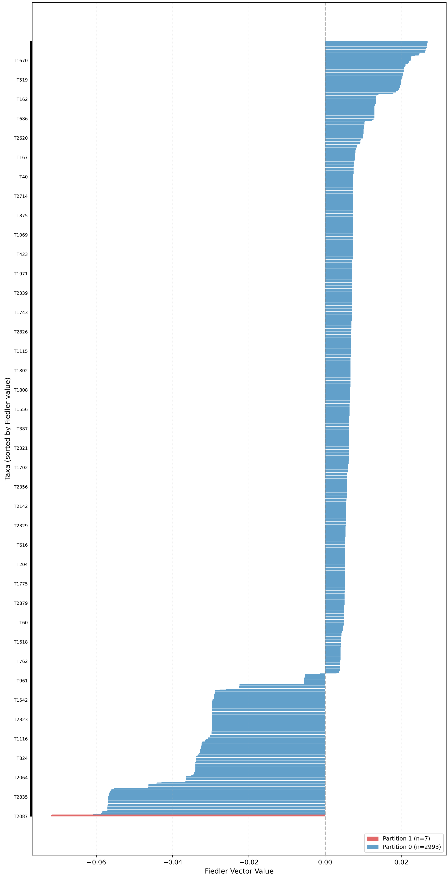
Partition for yule_pure_birth (n=3000, L=10000, \mu=0.20 ) - Fiedler Vector \sigma_2=0.0000 , Gap=0.0000, Coherence=0.1837
