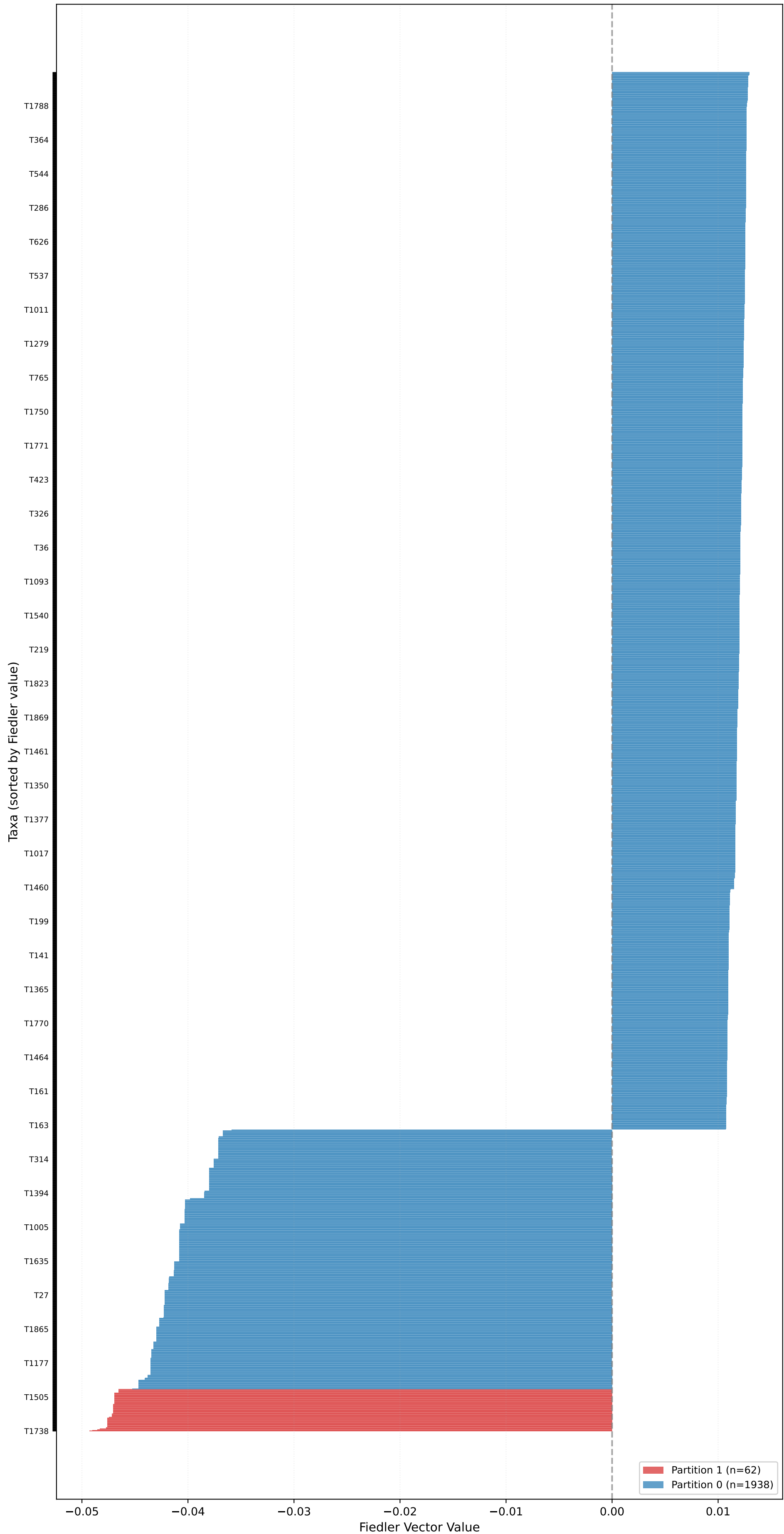
Partition for kingman_mean_pop_0.1 (n=2000, L=10000, \mu=0.10 ) - Fiedler Vector \sigma_2=0.0370 , Gap=48.5742, Coherence=0.0018
