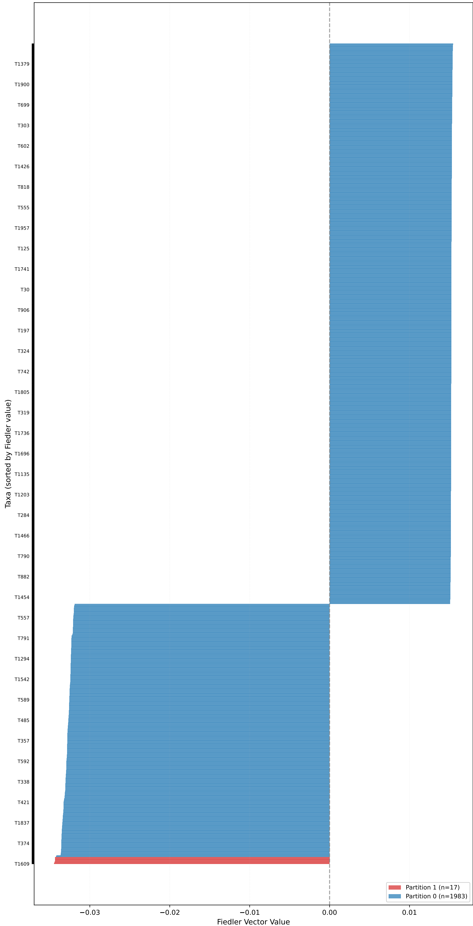
Partition for kingman_mean_pop_1 (n=2000, L=10000, \mu=0.10 ) - Fiedler Vector \sigma_2=0.0251 , Gap=154.7334, Coherence=0.0018
