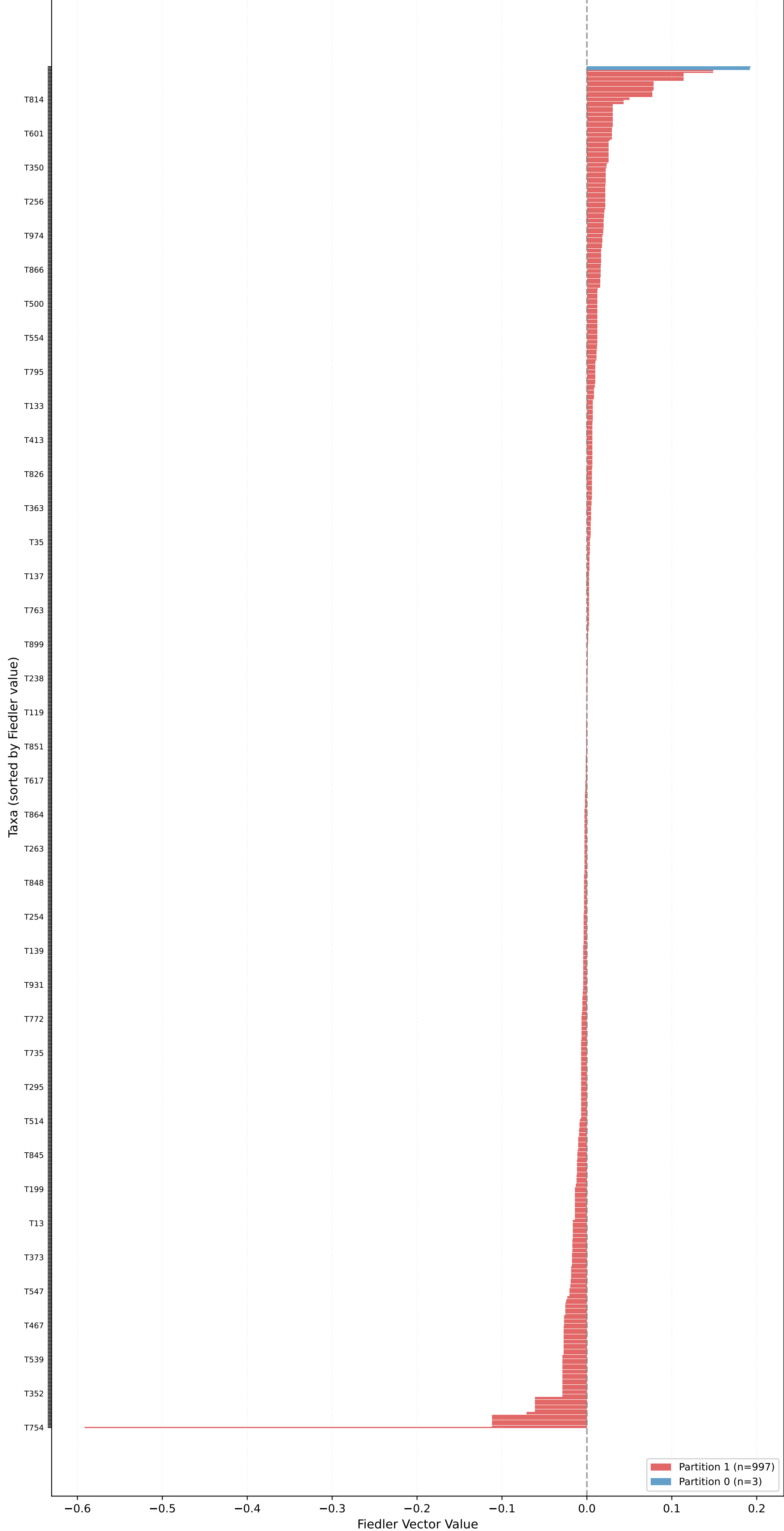
Partition for kingman_mean_pop_1000 (n=1000, L=10000, \mu=0.10 ) - Fiedler Vector \sigma_2=0.0000 , Gap=0.0000, Coherence=0.1448
