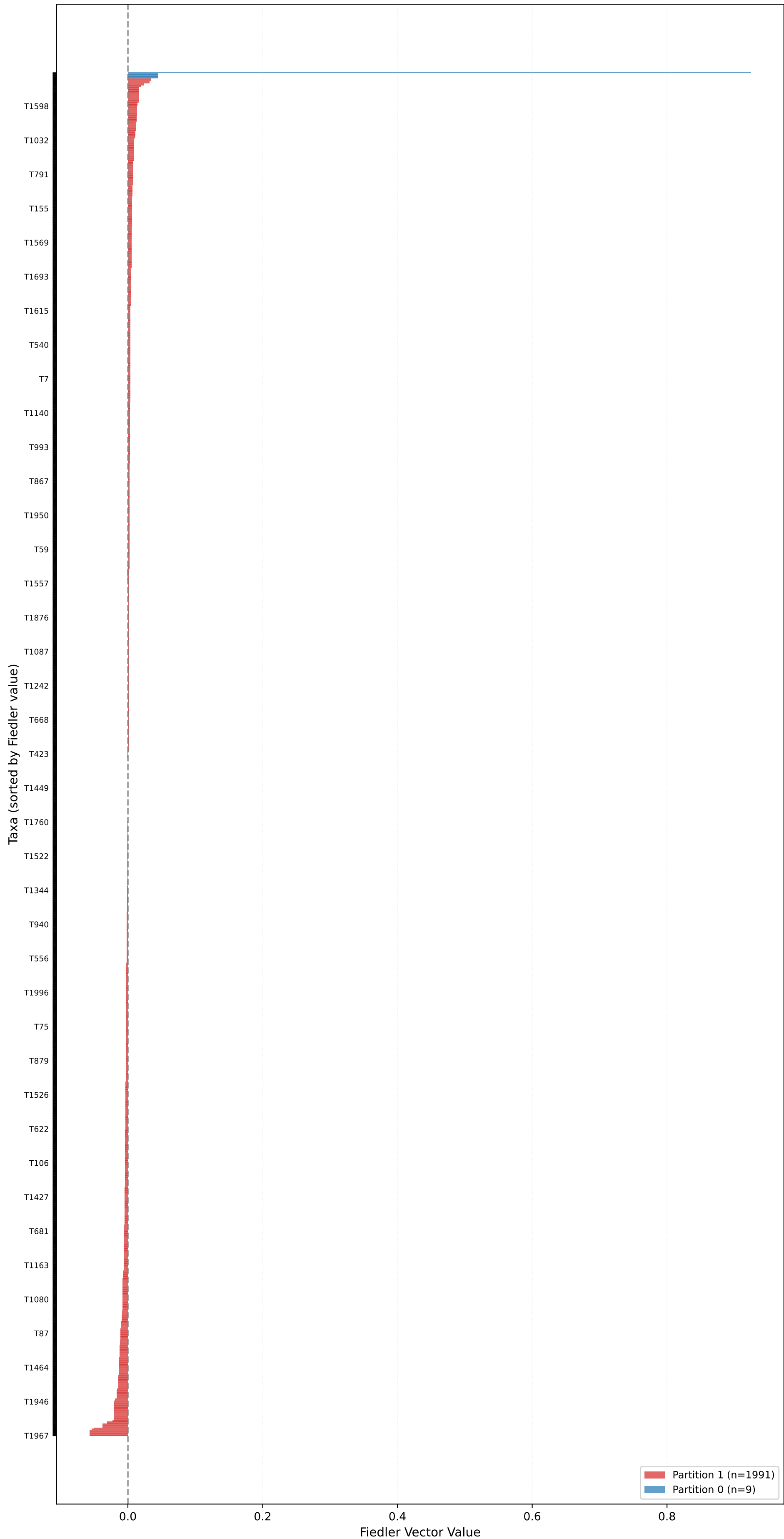
Partition for kingman_mean_pop_1000 (n=2000, L=10000, \mu=0.20 ) - Fiedler Vector \sigma_2=0.0000 , Gap=0.0000, Coherence=0.1467
