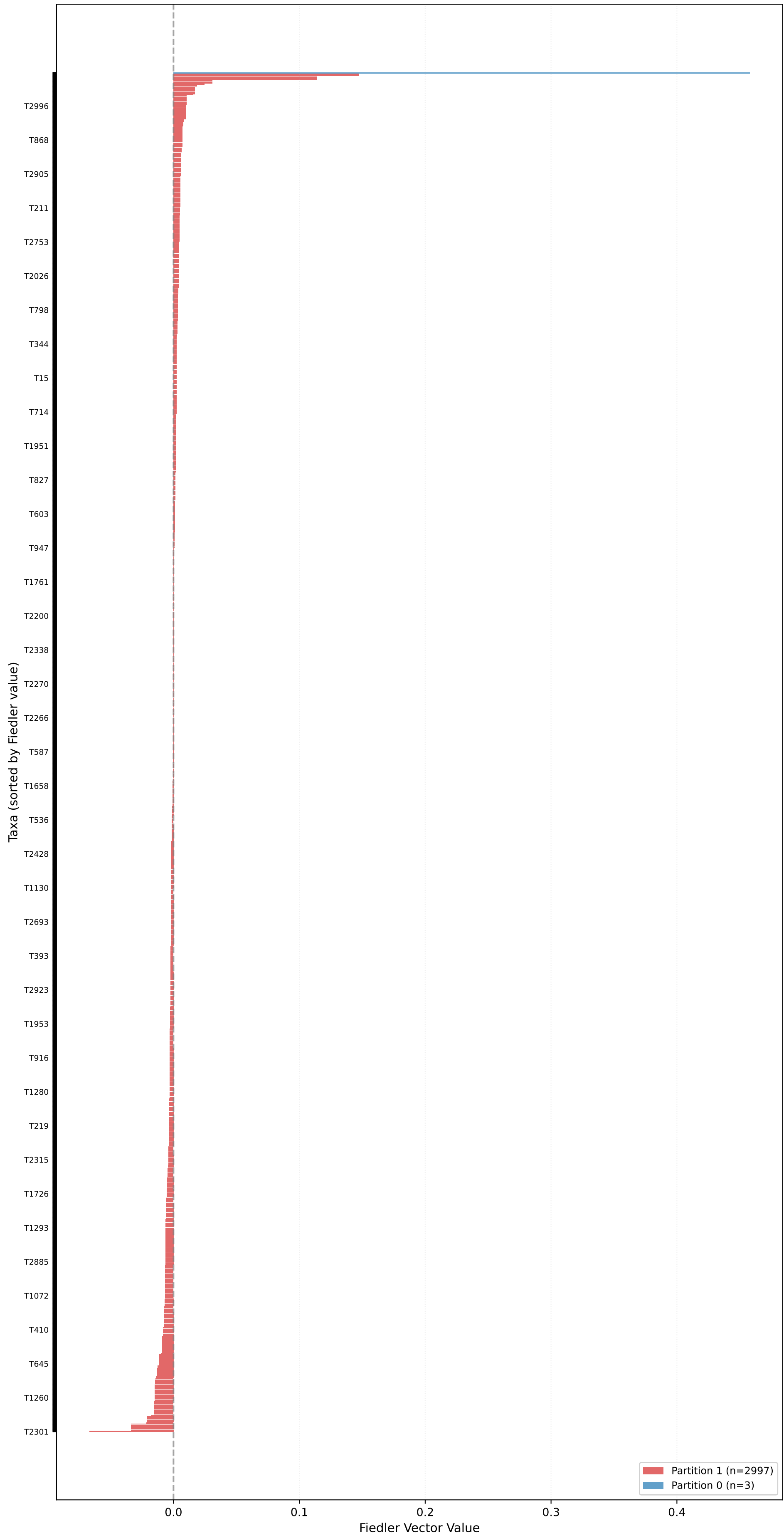
Partition for kingman_mean_pop_1000 (n=3000, L=10000, \mu=0.10 ) - Fiedler Vector \sigma_2=0.0000 , Gap=0.0000, Coherence=0.0775
