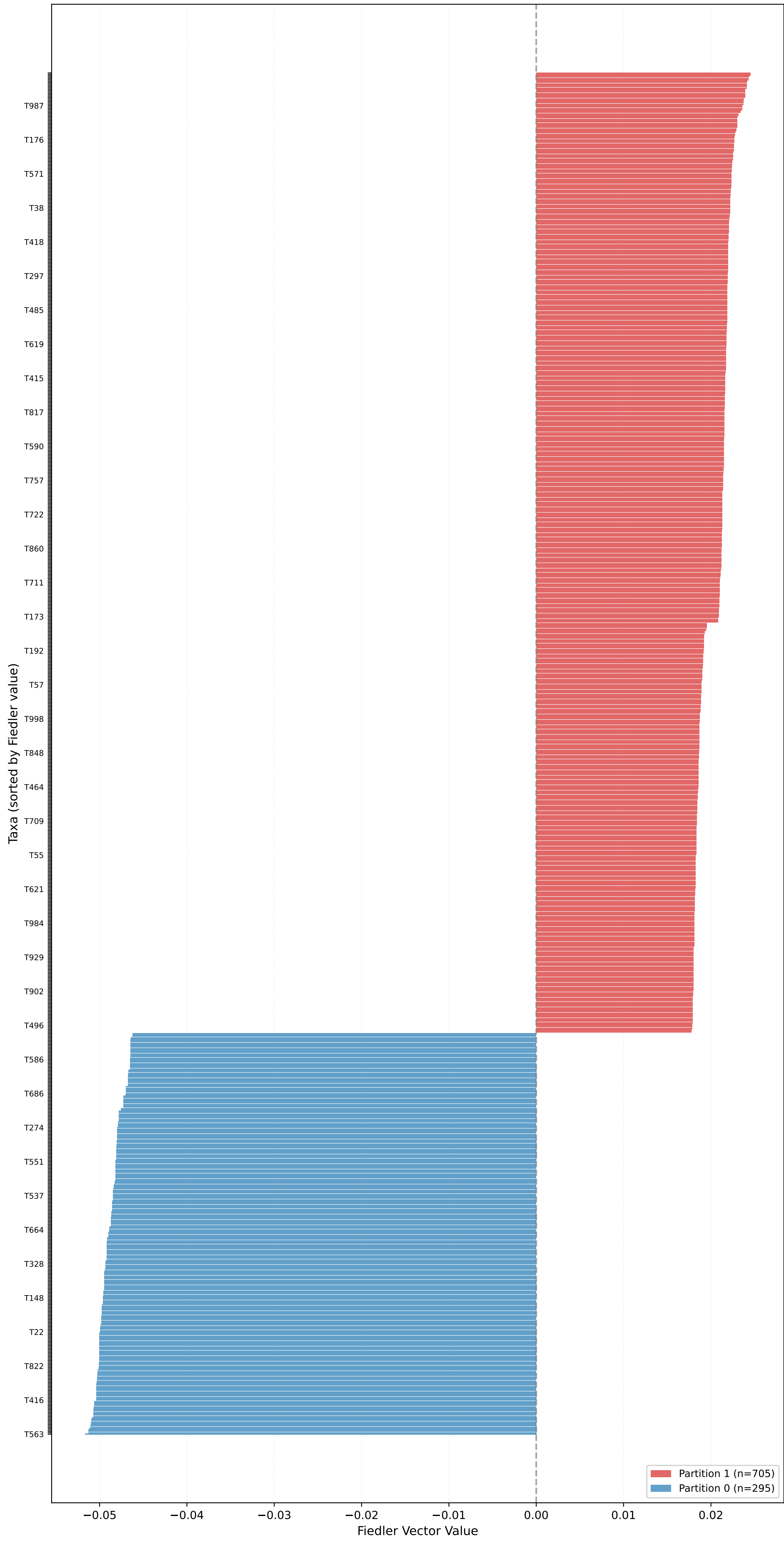
Partition for unrooted_pure_kingman_tree_pop_size_0.1 (n=1000, L=10000, \mu=0.20 ) - Fiedler Vector \sigma_2=0.1484 , Gap=16.2970, Coherence=0.0025
