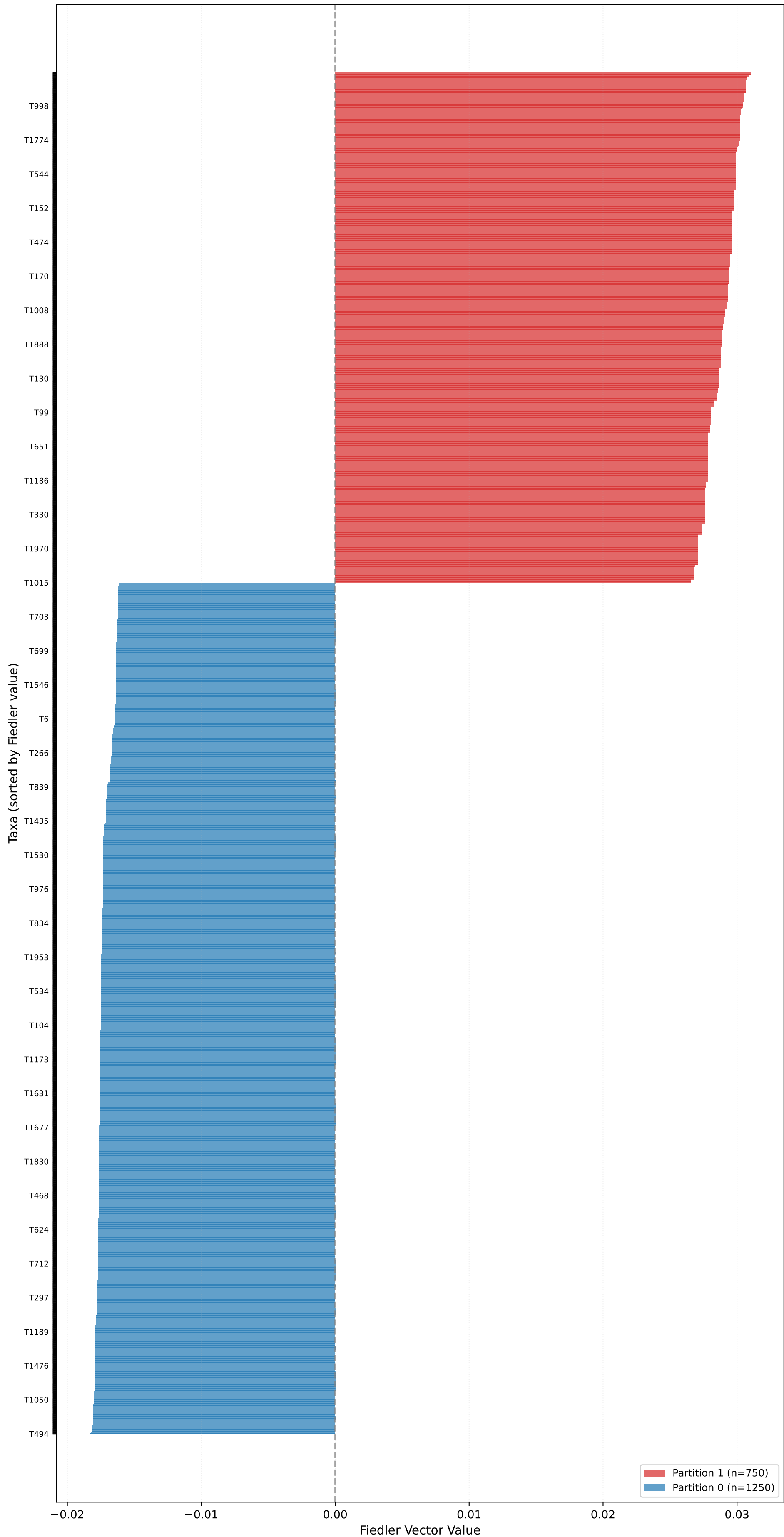
Partition for unrooted_pure_kingman_tree_pop_size_0.1 (n=2000, L=10000, \mu=0.10 ) - Fiedler Vector \sigma_2=0.1815 , Gap=51.3224, Coherence=0.0010
