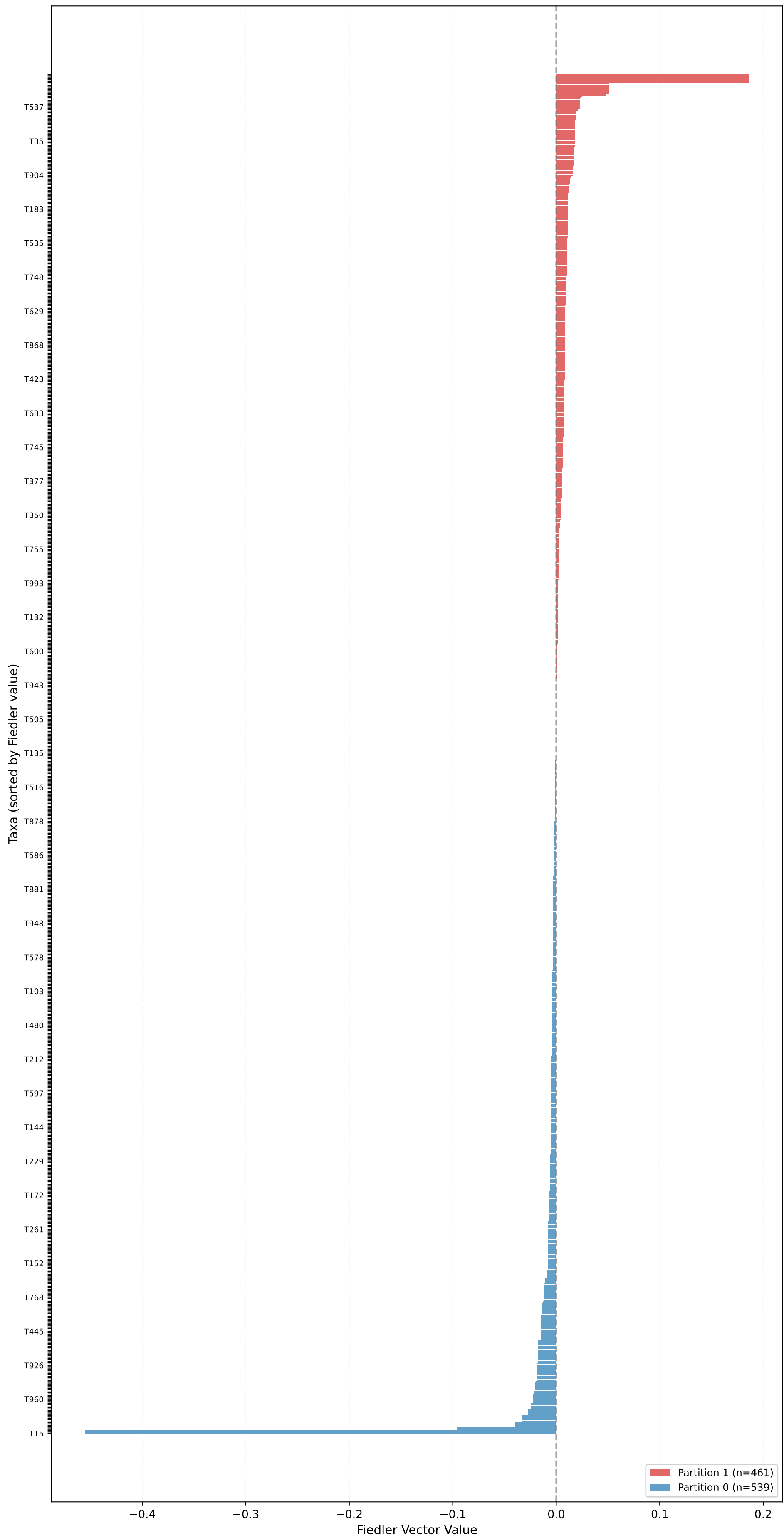
Partition for unrooted_pure_kingman_tree_pop_size_1000 (n=1000, L=10000, \mu=0.10 ) - Fiedler Vector \sigma_2=0.0001 , Gap=0.0000, Coherence=0.1547
