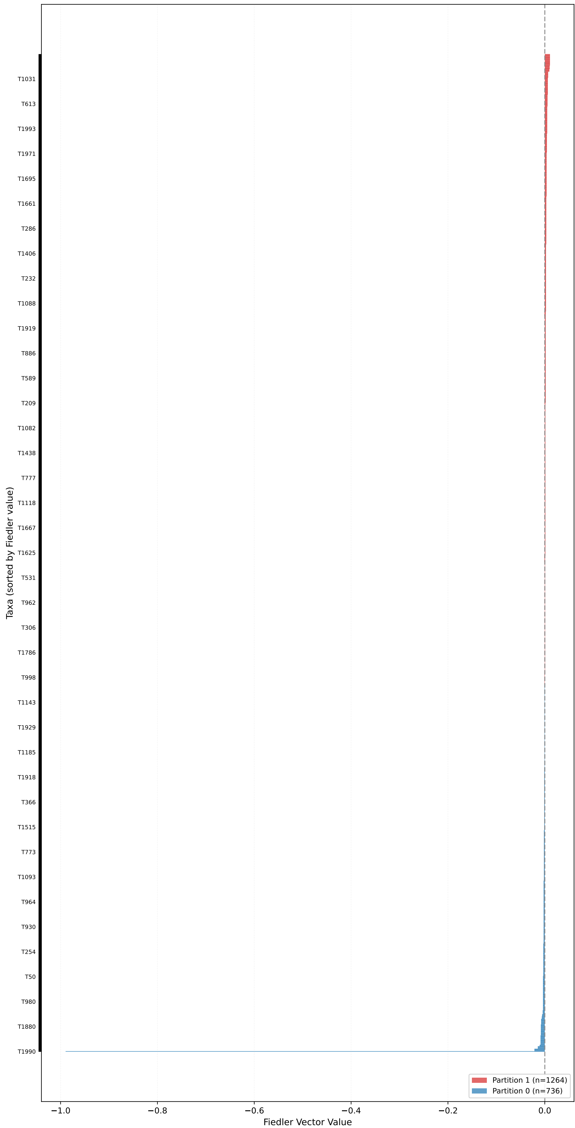
Partition for unrooted_pure_kingman_tree_pop_size_1000 (n=2000, L=10000, \mu=0.10 ) - Fiedler Vector \sigma_2=0.0002 , Gap=0.0000, Coherence=0.1081
