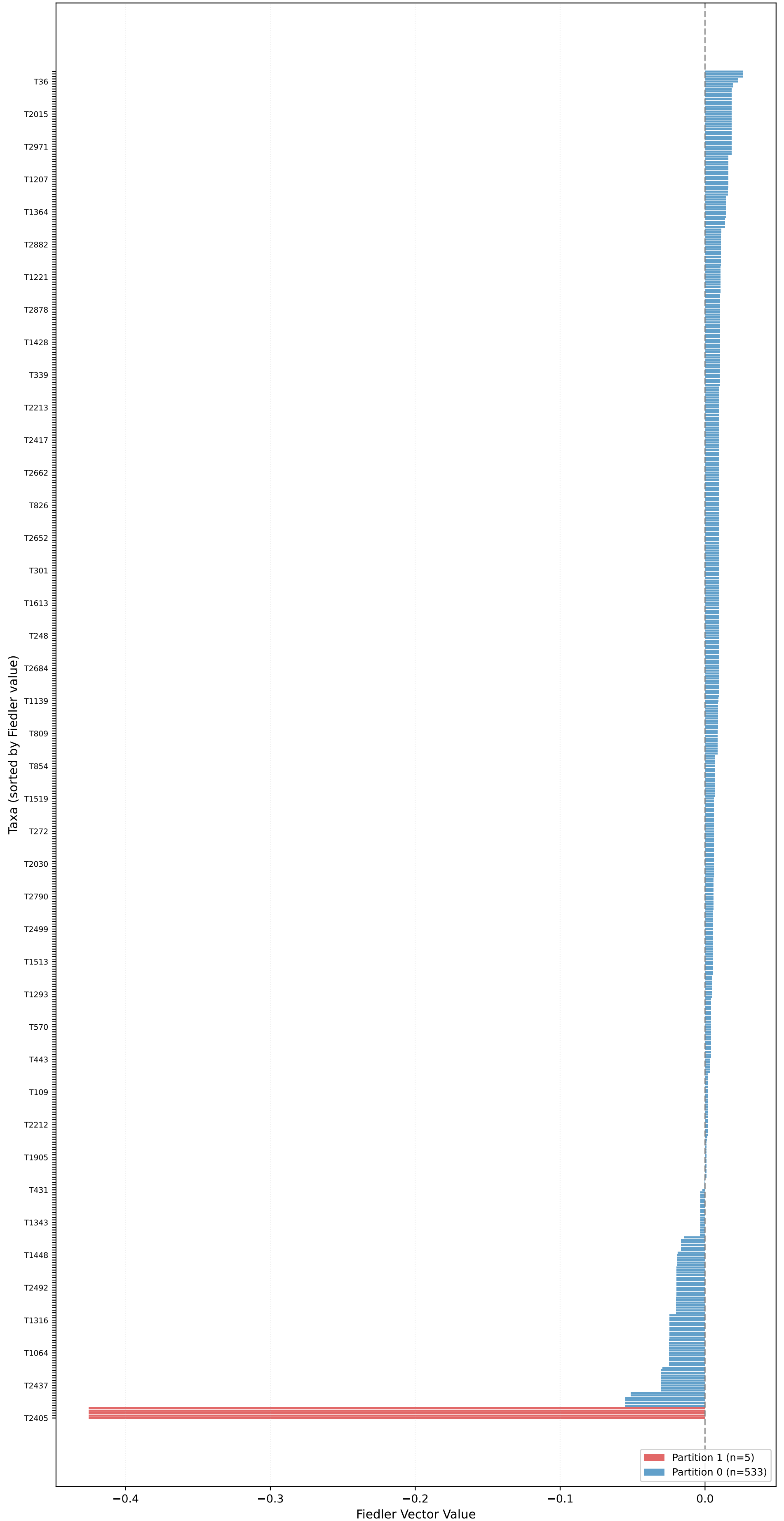
Partition for extinction_heavy (n=3000, L=10000, \mu=0.10 ) - Fiedler Vector \sigma_2=0.0000 , Gap=0.0000, Coherence=0.1467
