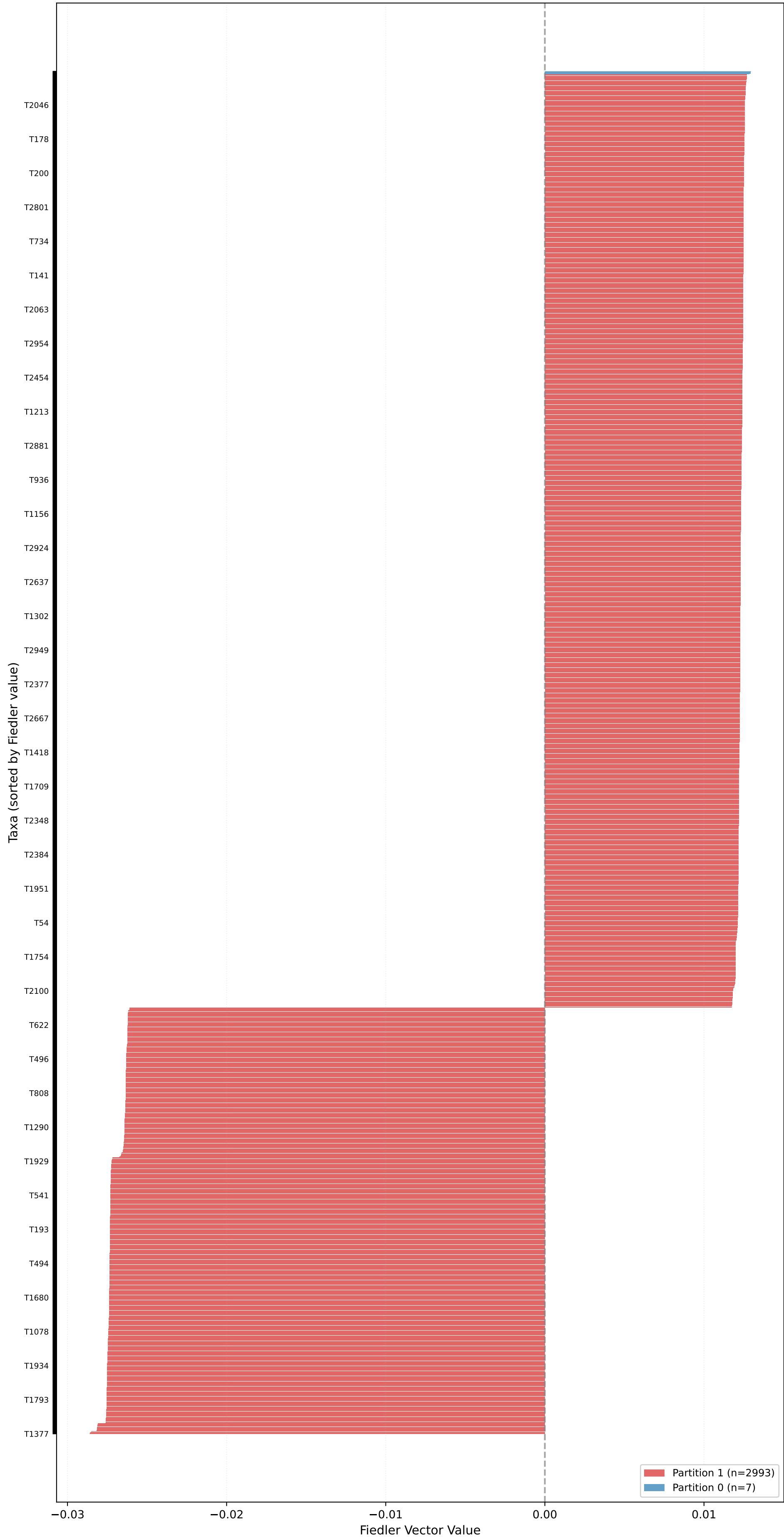
Partition for yule_pure_birth (n=3000, L=10000, \mu=0.10 ) - Fiedler Vector \sigma_2=0.0006 , Gap=0.0053, Coherence=0.1123
