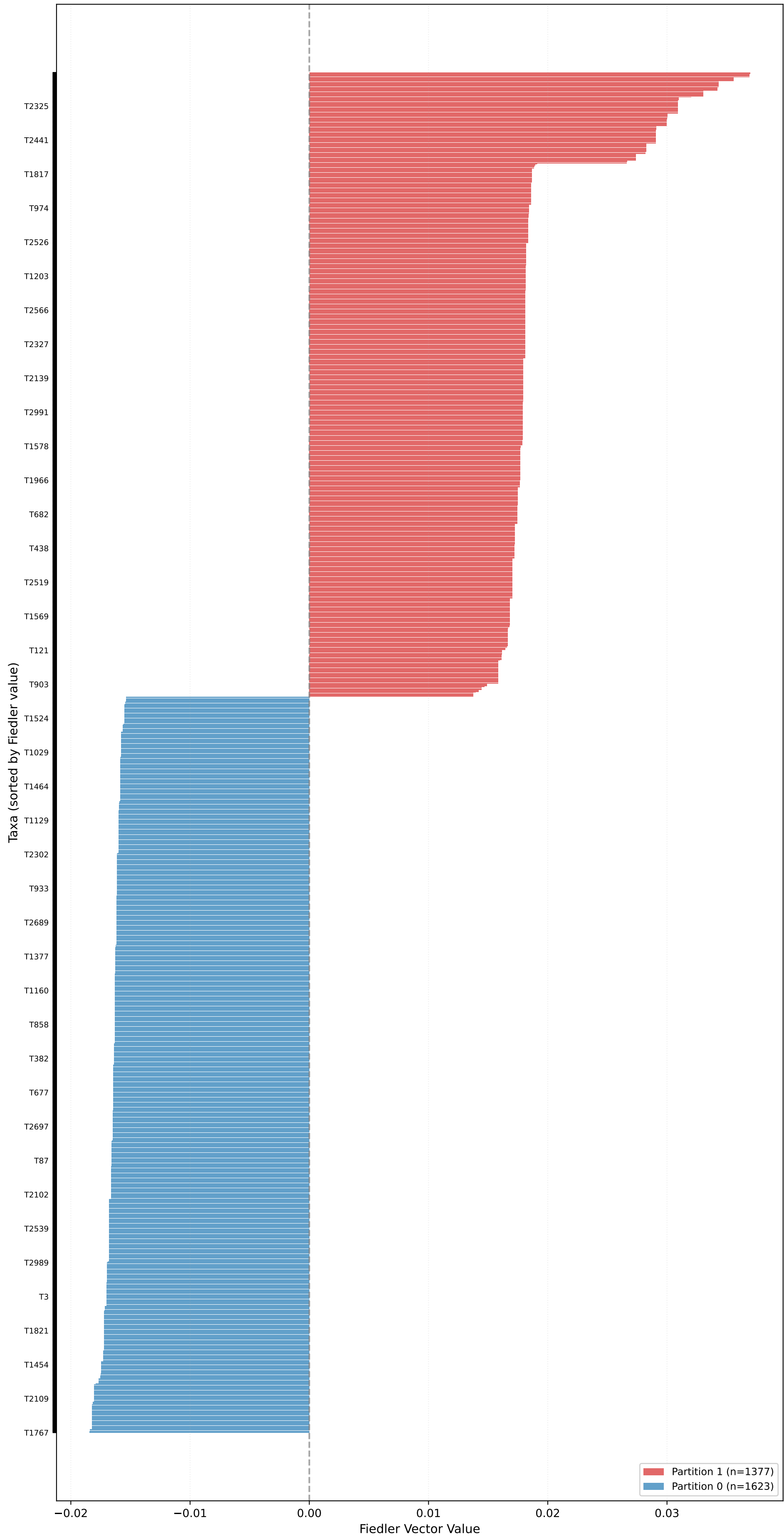
Partition for unrooted_pure_kingman_tree_pop_size_0.1 (n=3000, L=10000, \mu=0.10 ) - Fiedler Vector \sigma_2=0.0945 , Gap=25.2757, Coherence=0.0005
