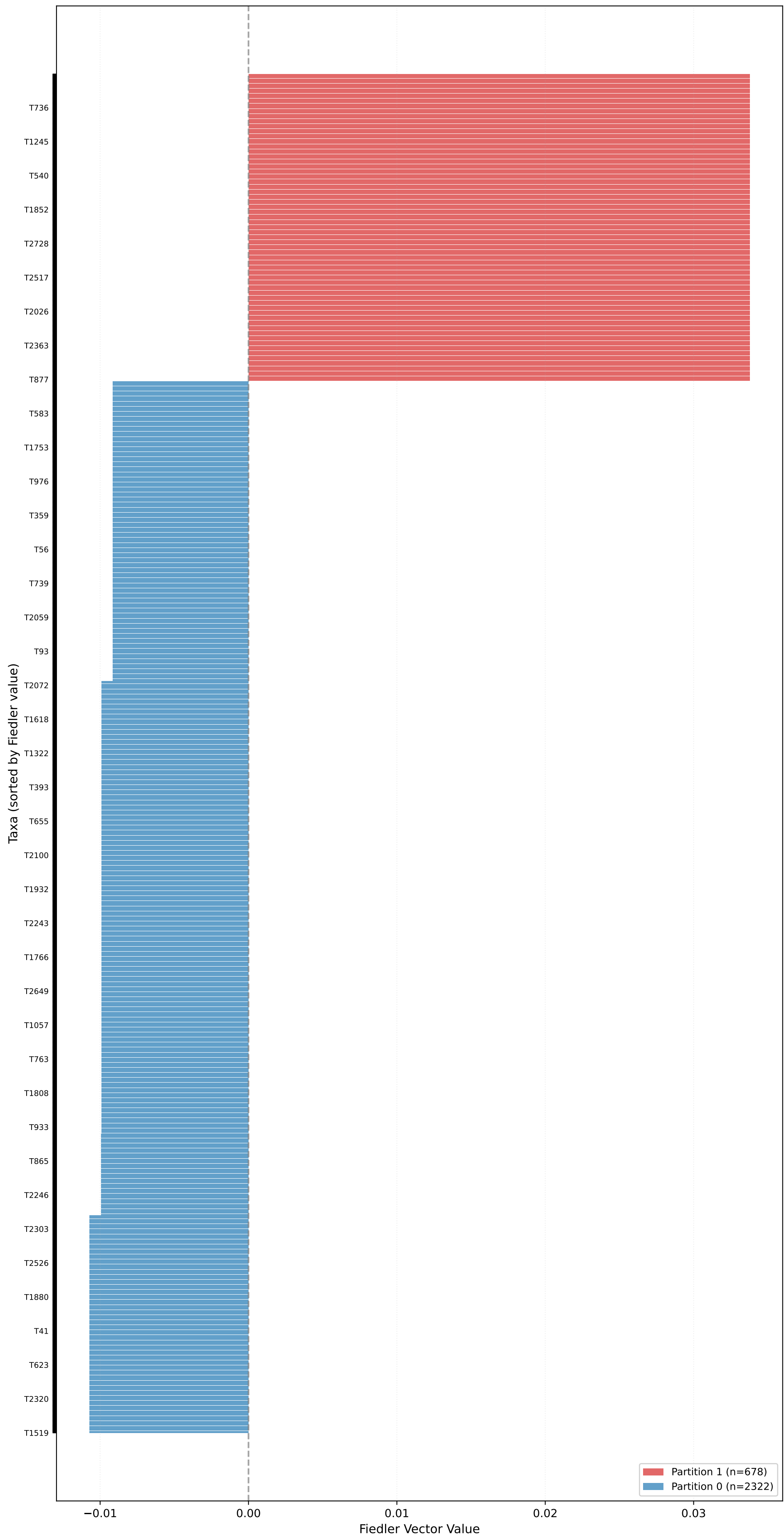
Partition for unrooted_kingman_tree_pop_size_10 (n=3000, L=10000, \mu=0.20 ) - Fiedler Vector \sigma_2=0.0002 , Gap=0.0005, Coherence=0.0029
