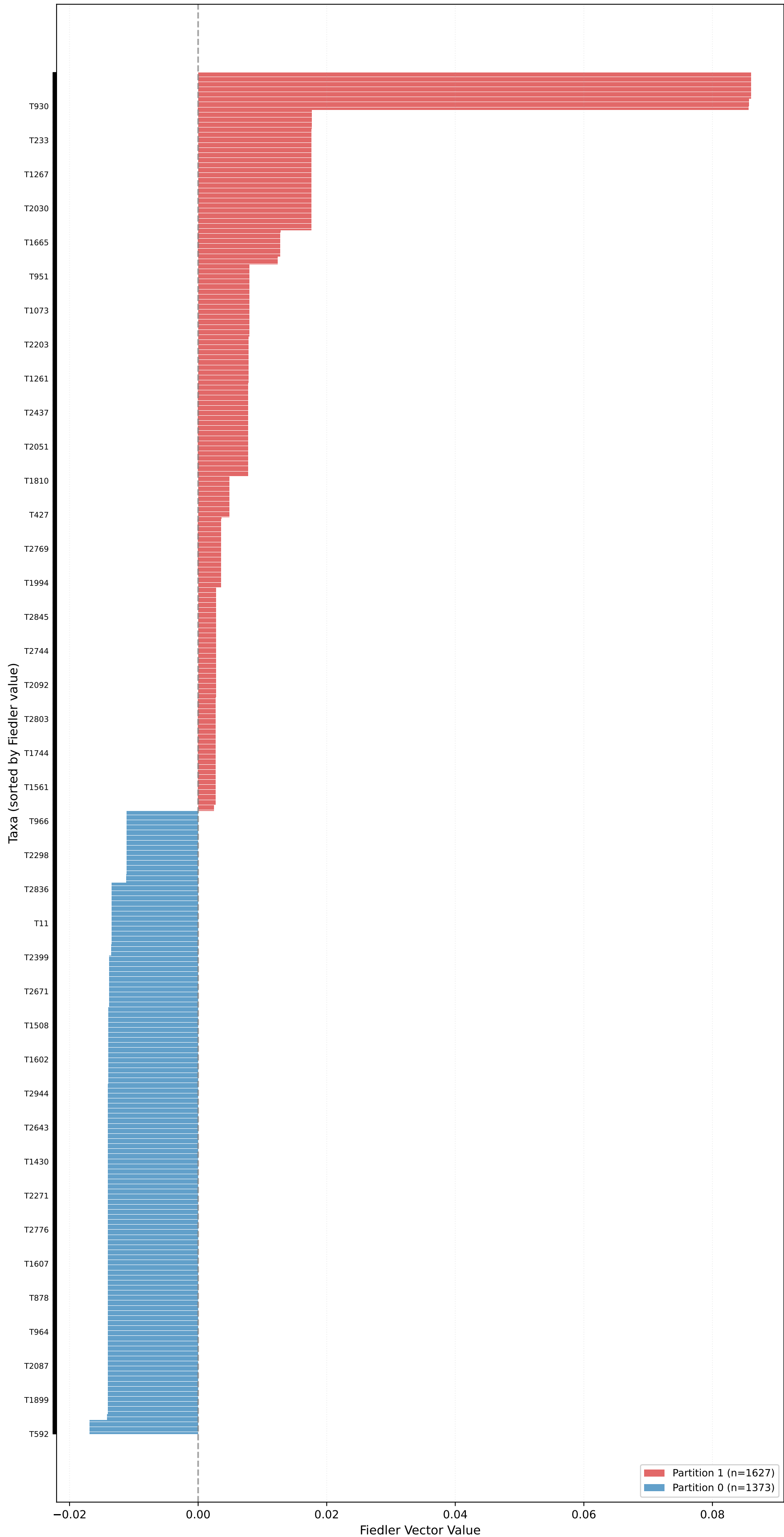
Partition for unrooted_pure_kingman_tree_pop_size_100 (n=3000, L=10000, \mu=0.10 ) - Fiedler Vector \sigma_2=0.0003 , Gap=0.0000, Coherence=0.0140
