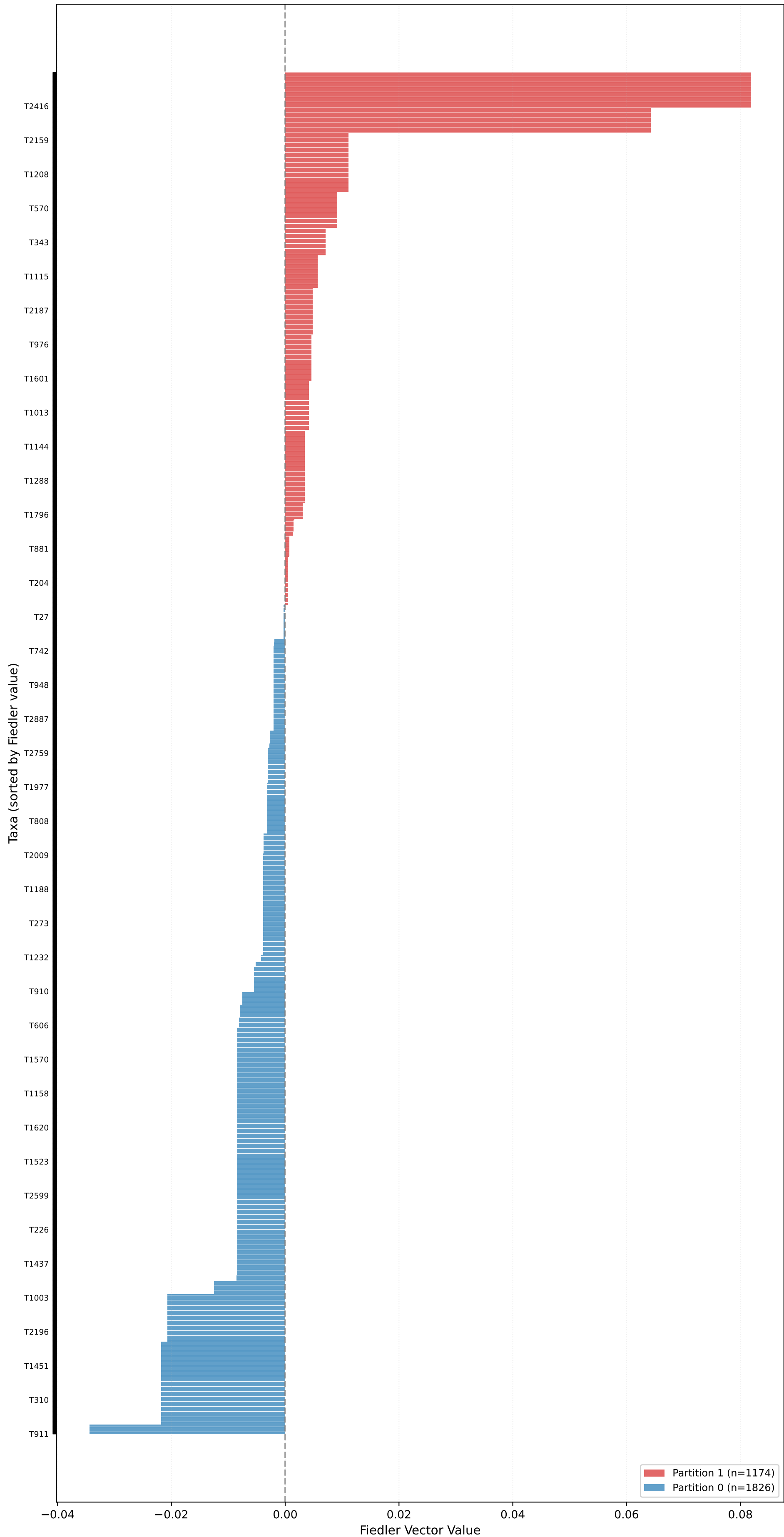
Partition for unrooted_pure_kingman_tree_pop_size_100 (n=3000, L=10000, \mu=0.20 ) - Fiedler Vector \sigma_2=0.0003 , Gap=0.0001, Coherence=0.0150
