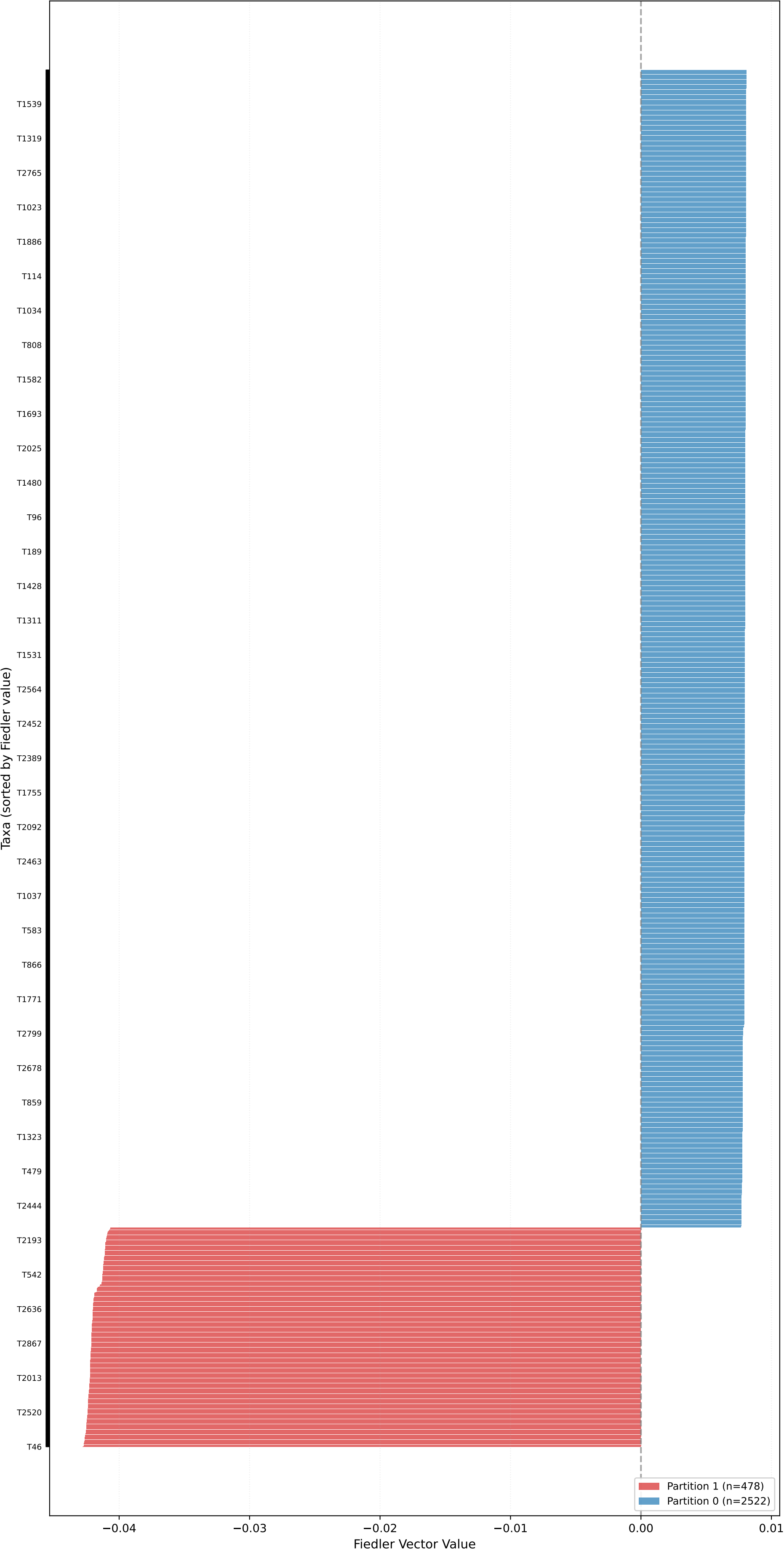
Partition for kingman_mean_pop_1 (n=3000, L=10000, \mu=0.10 ) - Fiedler Vector \sigma_2=0.4500 , Gap=184.7092, Coherence=0.0022
