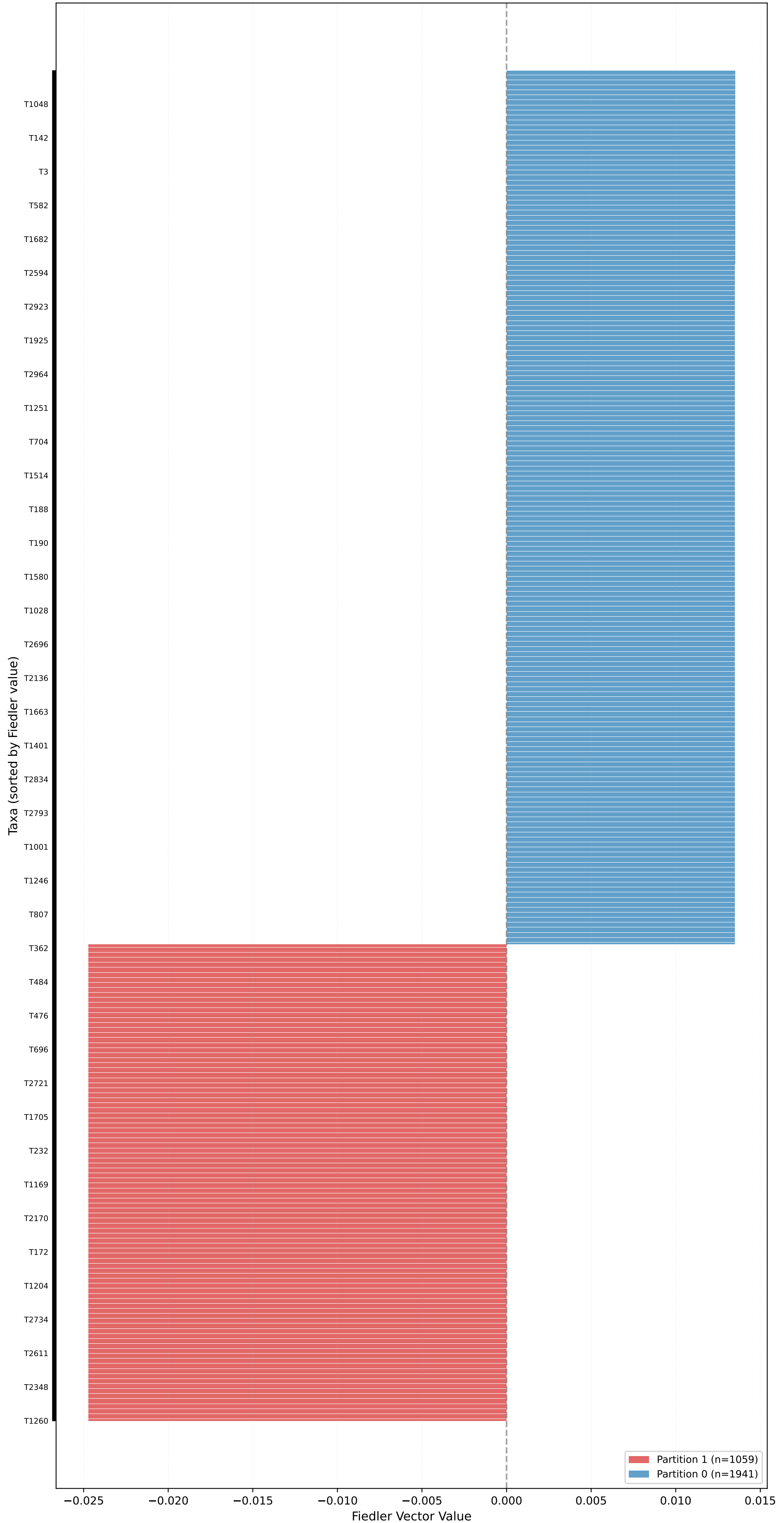
Partition for kingman_mean_pop_10 (n=3000, L=10000, \mu=0.10 ) - Fiedler Vector \sigma_2=0.0002 , Gap=0.6678, Coherence=0.0023
