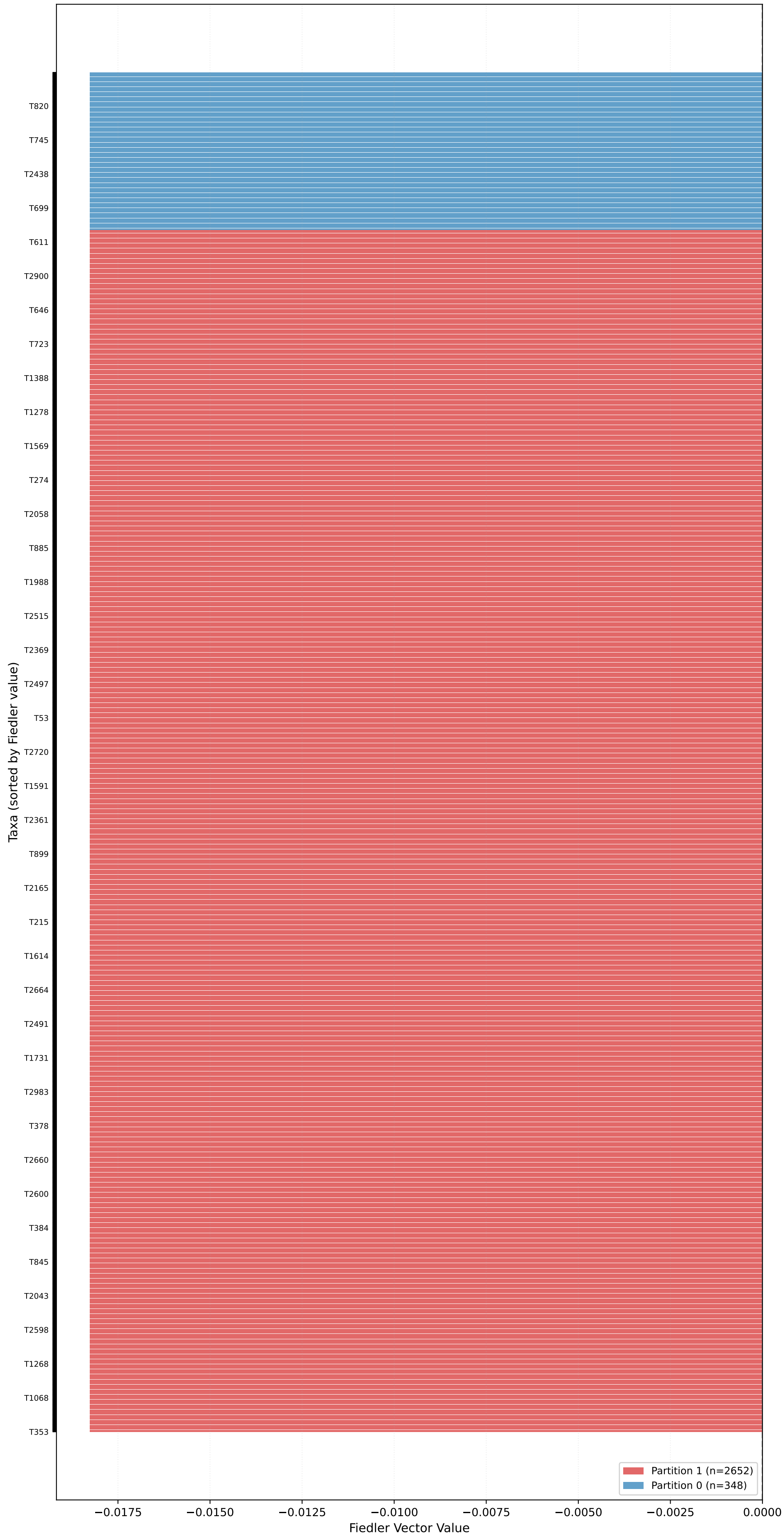
Partition for kingman_mean_pop_10 (n=3000, L=10000, \mu=0.20 ) - Fiedler Vector \sigma_2=0.0002 , Gap=0.0007, Coherence=0.0042
